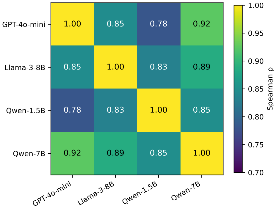
Cross-model Spearman correlation (subject-level ECE, 57 subjects)
