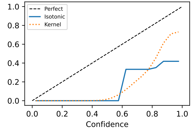
Virology ECE=0.427
