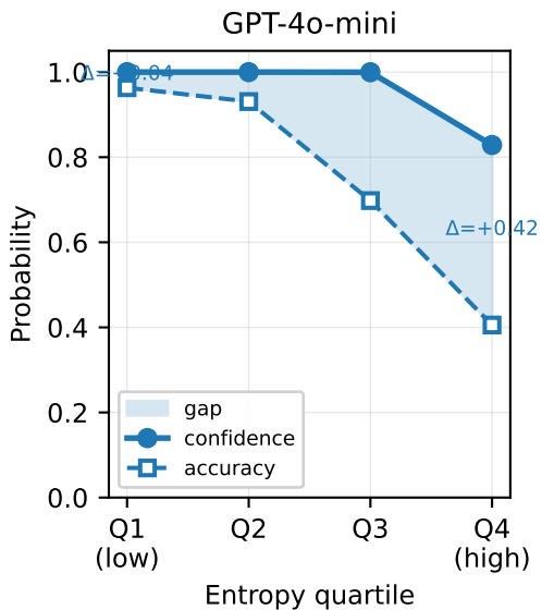
Confidence vs. accuracy by entropy quartile per model (shaded = calibration gap)
