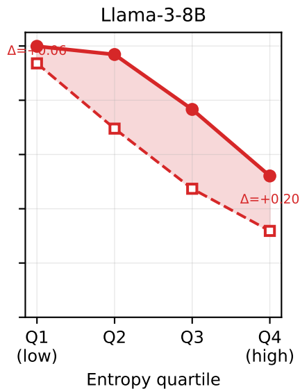
Confidence vs. accuracy by entropy quartile per model (shaded = calibration gap)
