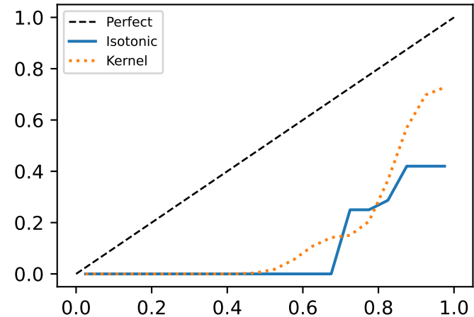
virology ECE=0.432
