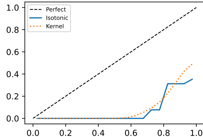
formal_logic ECE=0.390
