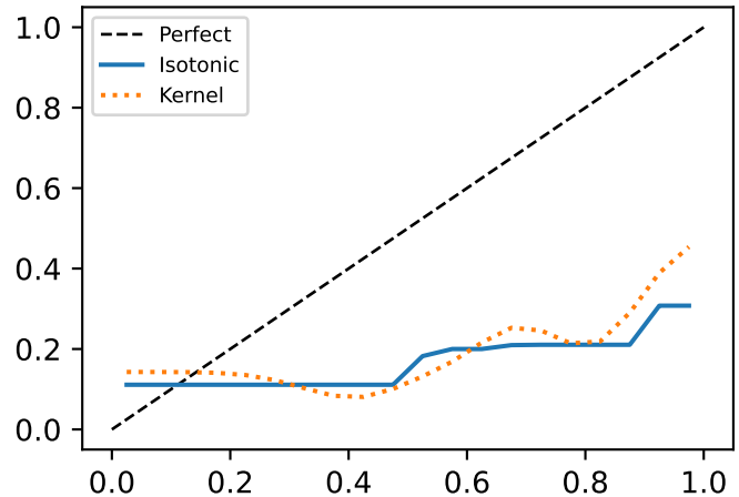
abstract_algebra ECE=0.426
