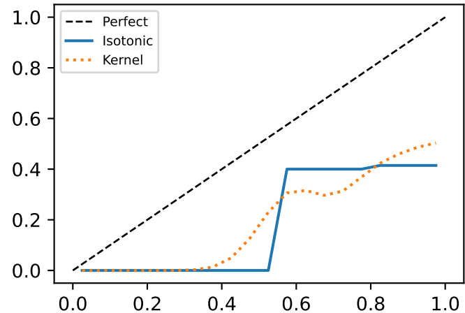
global_facts ECE=0.401
