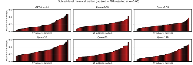
Figure 6. Mean calibration gap per subject, sorted ascending, for the six larger models (Qwen-0.5B omitted; see Section 3.3). Red bars are FDR-rejected at \alpha = 0.05 ; gray bars are not. Five of six models reject all 57 subjects; Qwen-1.5B (fp16) rejects 56/57.
