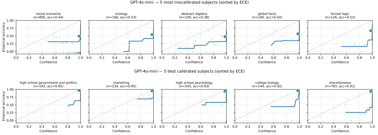
Figure 1. GPT-4o-mini reliability curves. Top: five most miscalibrated subjects by ECE. Bottom: five best-calibrated subjects. Same conventions in both: solid line is isotonic regression, plotted only on observed support; markers are 20-bin empirical accuracy sized by bin count; dashed line is the calibration diagonal.
