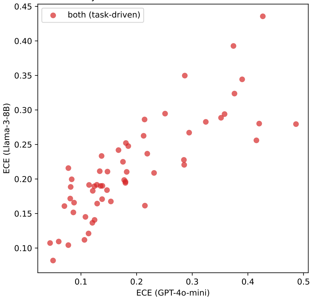
Subject ECE: GPT-4o-mini vs. Llama-3-8B
