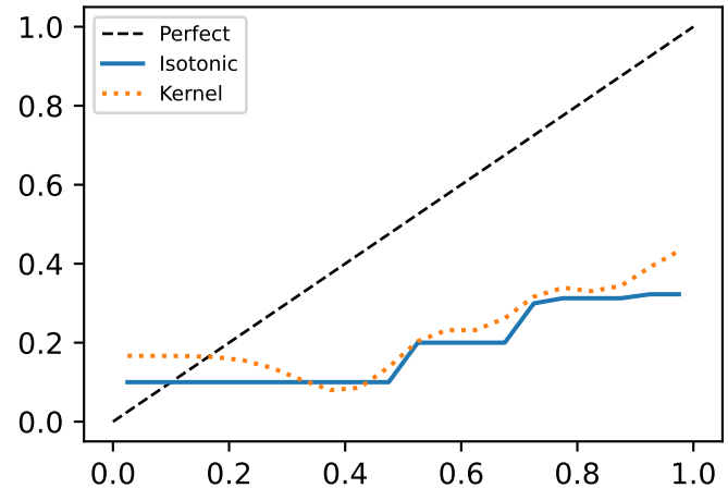
abstract_algebra ECE=0.420
