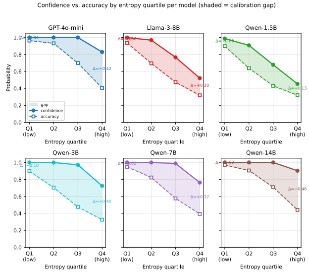
Figure 4. Confidence (solid) and accuracy (dashed) by entropy quartile for the six larger models (Qwen-0.5B omitted; see Section 3.3). Shaded area is the calibration gap. Within Qwen, the curves move roughly together at 1.5B, but separate progressively at 7B and 14B as confidence stays near saturation across quartiles while accuracy still falls with entropy.
