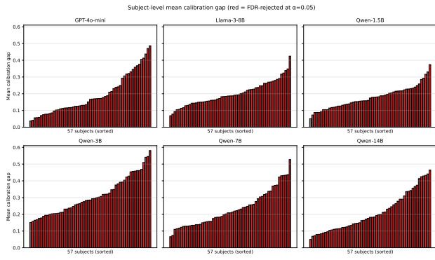
Figure 6. Mean calibration gap per subject, sorted ascending, for the six larger models (Qwen-0.5B omitted; see Section 3.3). Red bars are FDR-rejected at \alpha = 0.05 ; gray bars are not. Five of six models reject all 57 subjects; Qwen-1.5B (fp16) rejects 56/57.
