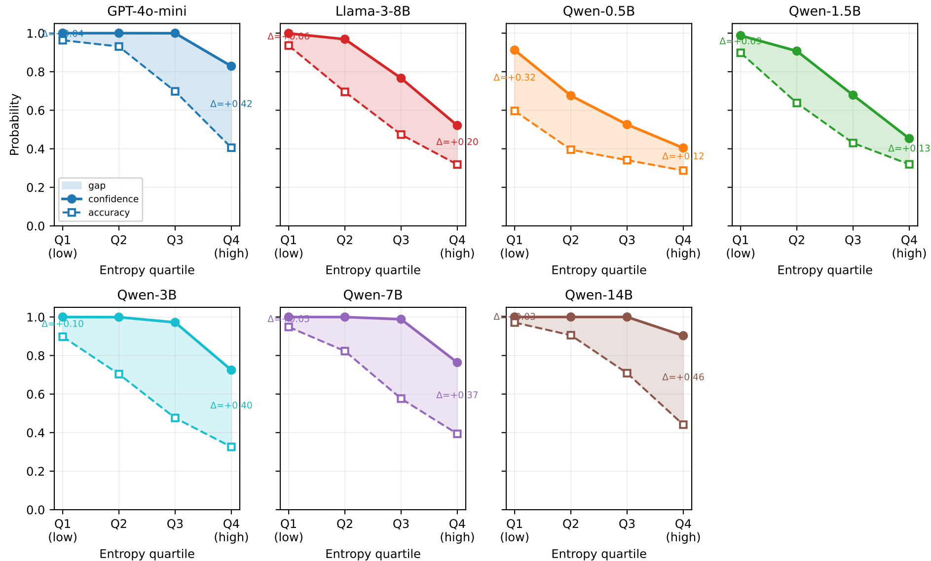
Confidence vs. accuracy by entropy quartile per model (shaded = calibration gap)
