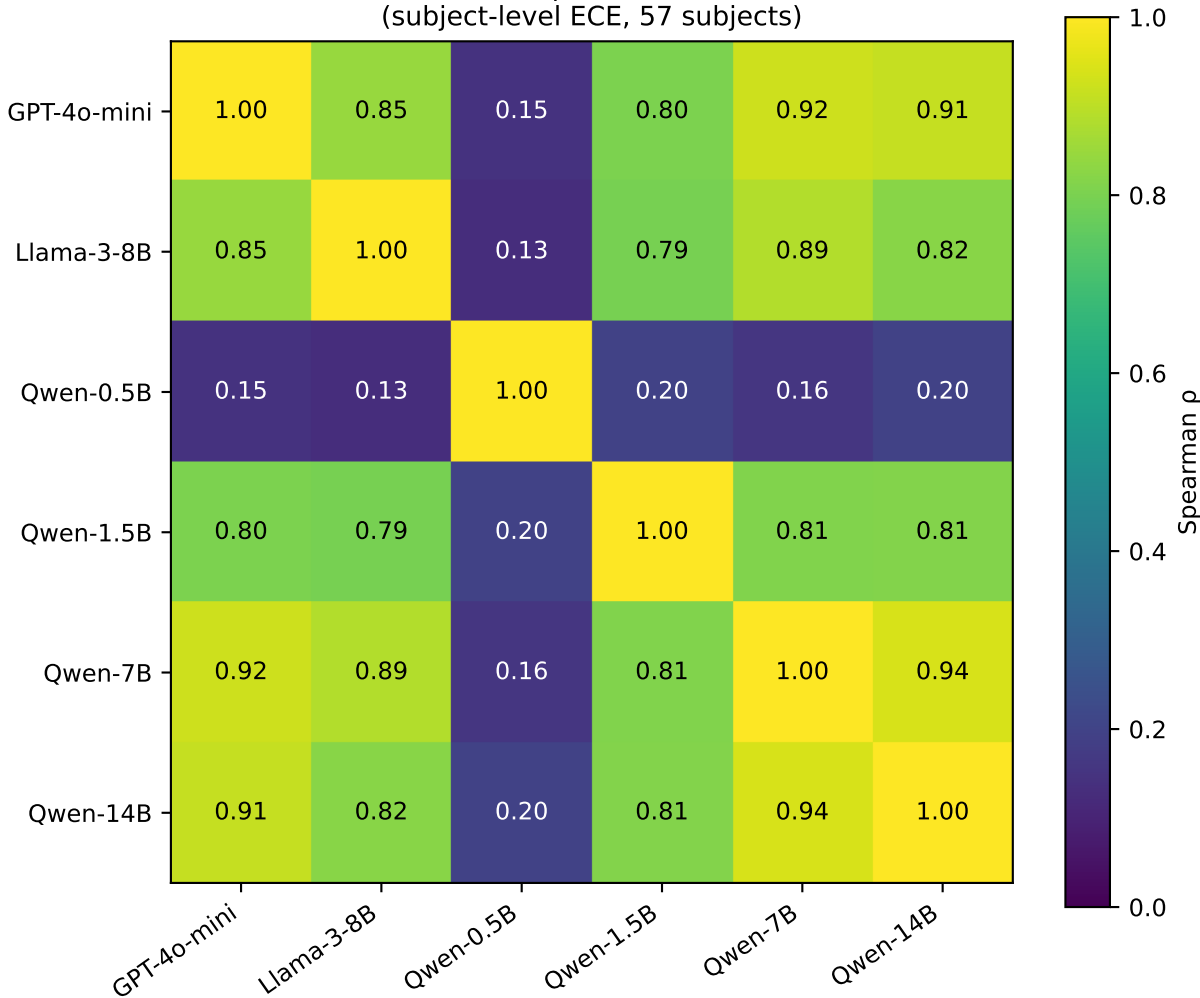
Cross-model Spearman correlation (subject-level ECE, 57 subjects)
