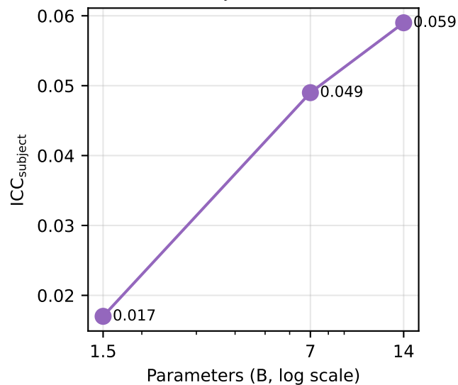
Between-subject variance share
