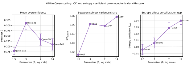
Figure 5. Within-Qwen scaling on the four matched-precision checkpoints. The entropy coefficient rises monotonically with scale; ICC jumps from 1.5B to 3B and then plateaus; the intercept is non-monotonic.
