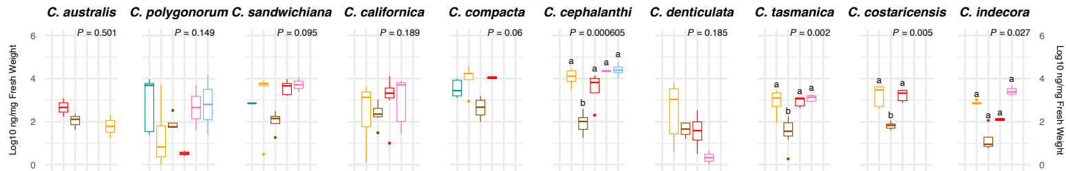
Chlorophyll a
