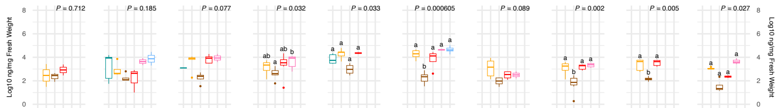
Total chlorophyll
