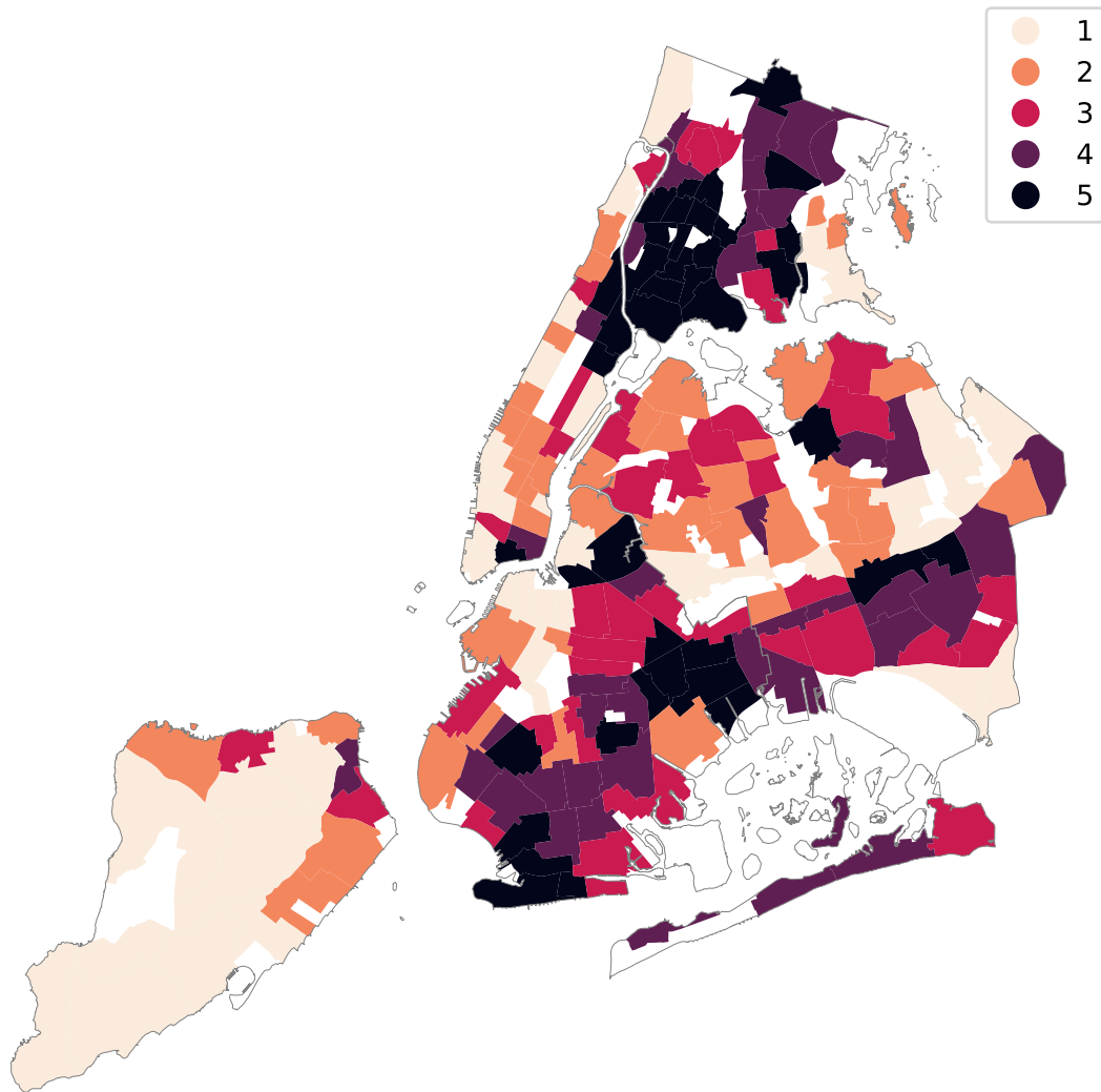
HVI: prioritizing age and poverty status
