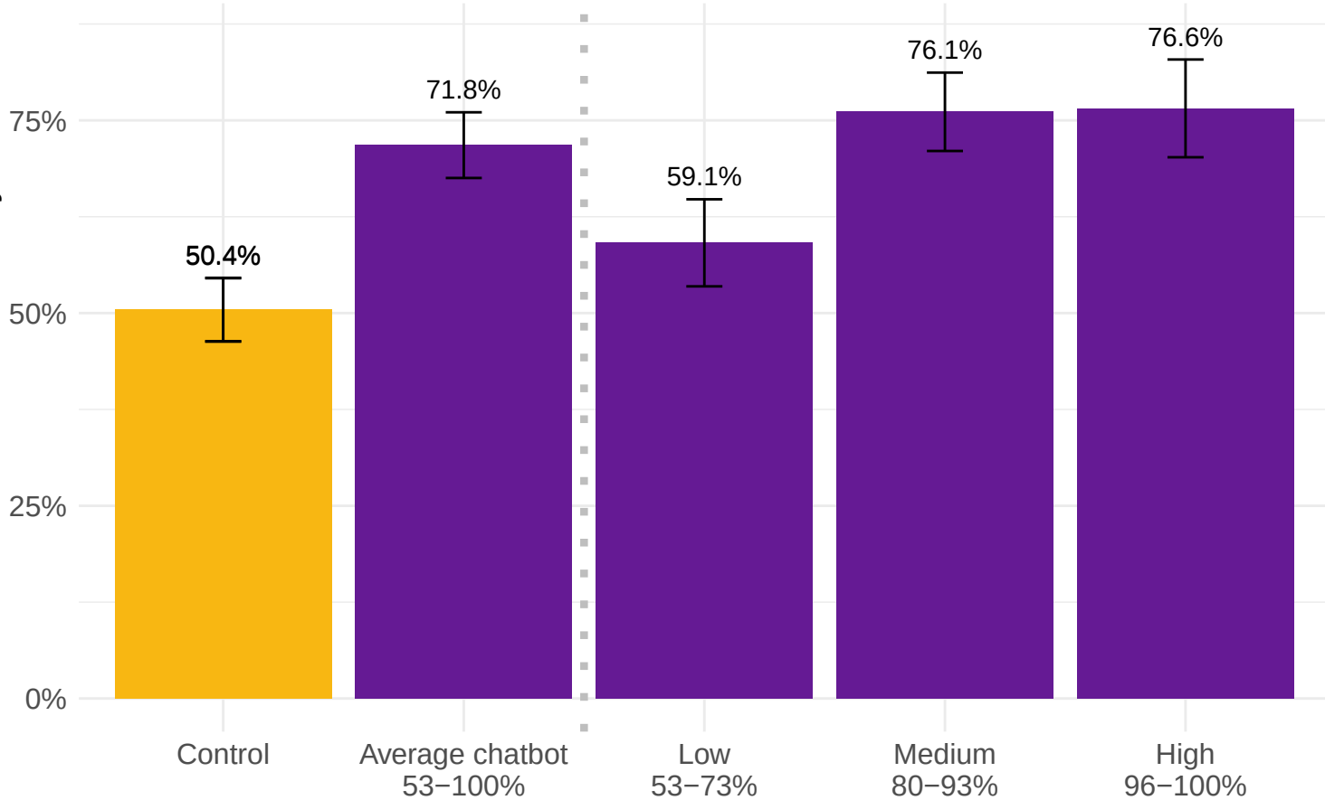
Caseworker accuracy
