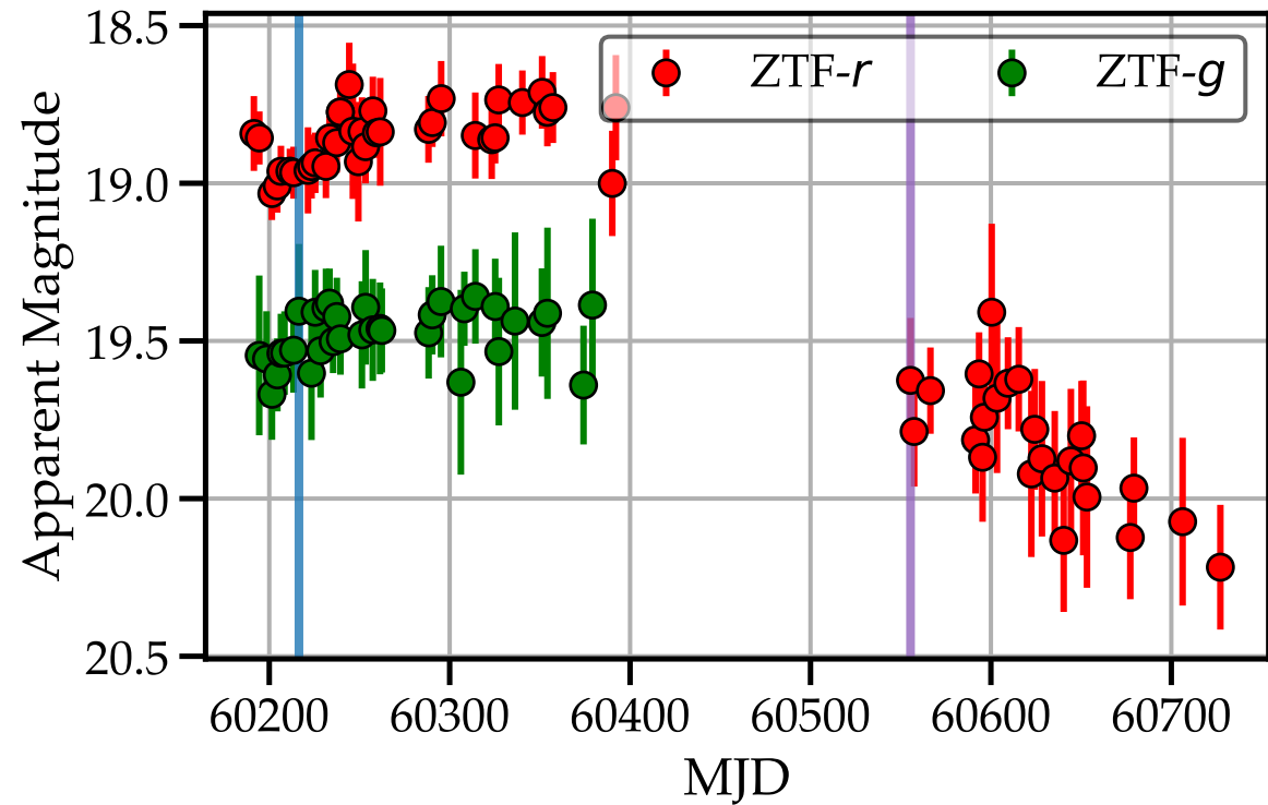
ZTF23abaeenk (SN II, z=0.035 ) [ p_{\max}(\text{Anomaly})=65.2\% ]
