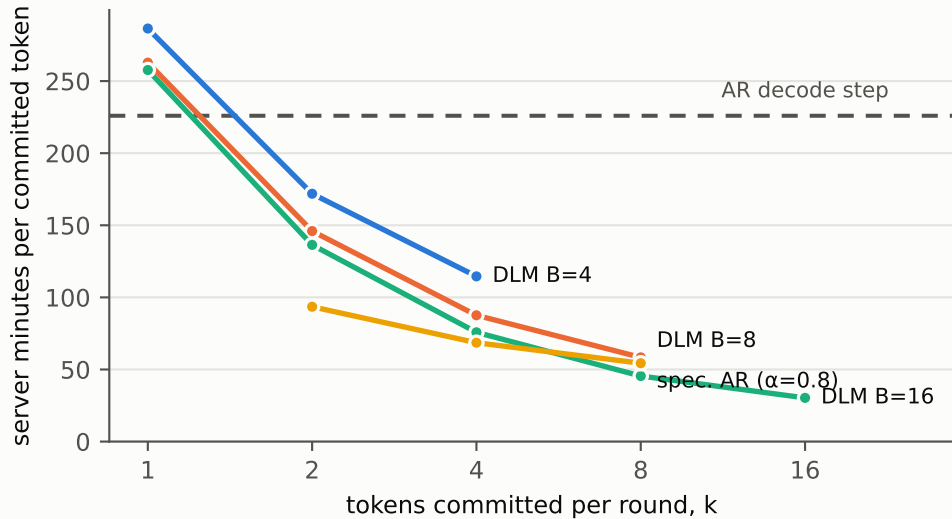
Encrypted cost per committed token (CPU OpenFHE, N=2^{17} )
