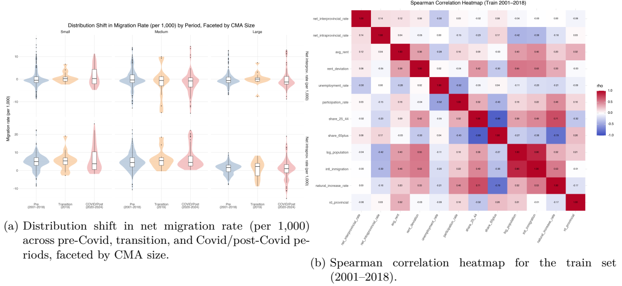
Figure 2: Period distribution shift by CMA size (left) and feature correlation heatmap on the training set (right).
