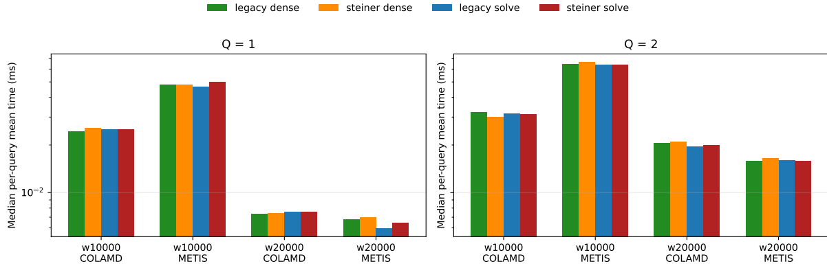
Figure 9: Baseline common queries remain in the same performance regime. For |\mathcal{Q}| = 1 and |\mathcal{Q}| = 2 on w10000 and w20000, all four variants cluster tightly on the log scale because these cases were already local in the pre-improvement implementation. The absolute difference between the two datasets reflects local Bayes-tree geometry near the sampled poses rather than the total graph size. Solve-based extraction yields only modest gains here, which is exactly why the much larger speedups in the later figures should be read as a correction to the older |\mathcal{Q}| > 2 path rather than as a blanket acceleration of every covariance query.
