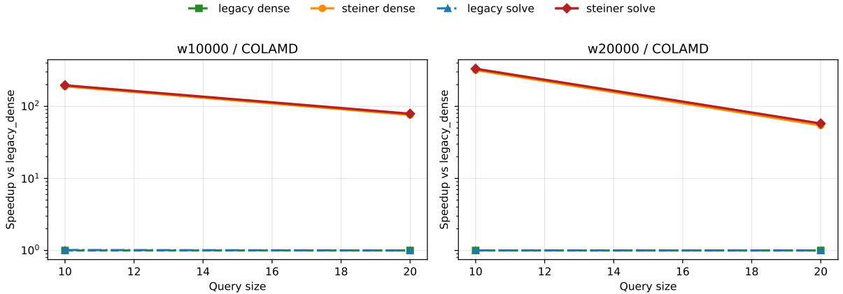
Figure 14: Solve-based extraction helps most on selected cross-covariance queries. Once Steiner localization has removed the global re-elimination cost, replacing dense inversion by selected triangular solves reduces the remaining extraction time and yields a modest but consistent total-time gain. This figure isolates the secondary numerical improvement more directly than the full-joint experiments.
