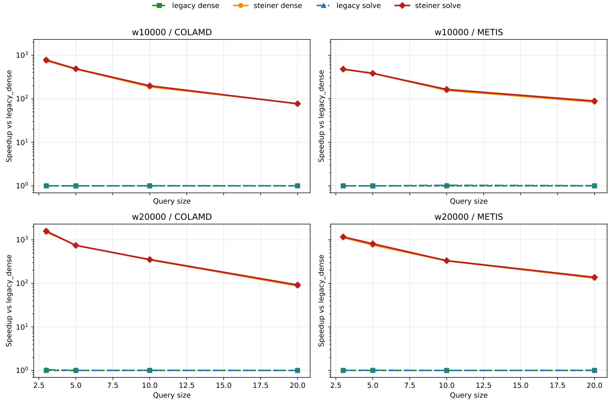
Figure 11: Steiner localization removes most of the cost for local joint covariances. For local windows on w10000 and w20000, both Steiner-based variants are faster than both pre-improvement variants by roughly two to three orders of magnitude, while the dense-versus-solve choice only changes the remaining small extraction cost. This figure shows that the new Steiner generalization is the main reason the method improves on the earlier implementation for larger joint queries.
