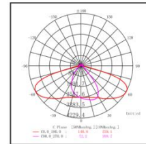
Polar Curve
