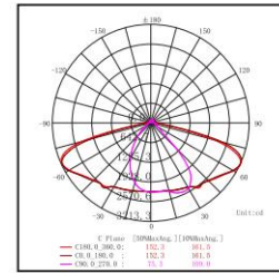
Polar Curve
