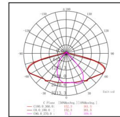
Polar Curve
