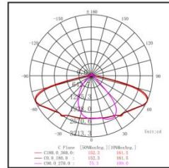
Polar Curve
