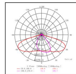
Polar Curve
