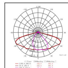
Polar Curve
