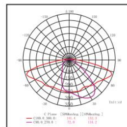
Polar Curve
