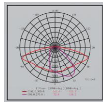
Polar Curve
