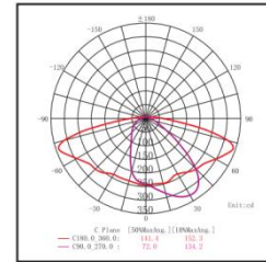
Polar Curve
