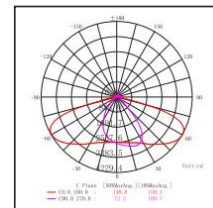
Polar Curve
