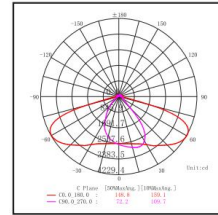
Polar Curve
