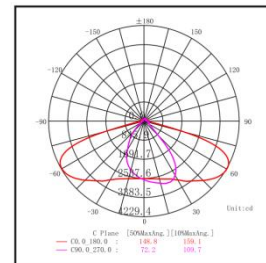
Polar Curve
