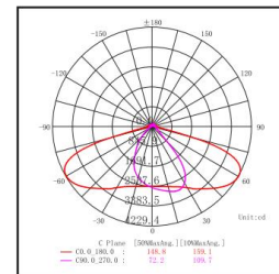
Polar Curve
