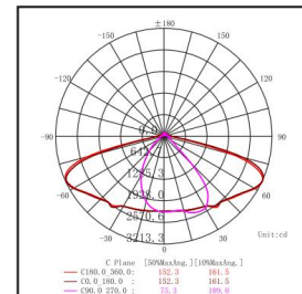
Polar Curve
