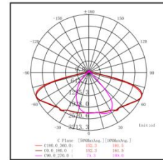
Polar Curve
