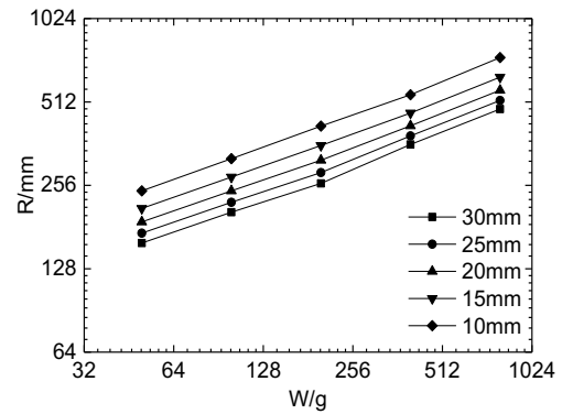
Fig.7 Iso-damage curve of cylinder
