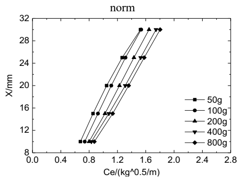
Fig.9 Iso-damage curve of circular plate under energy flux density
