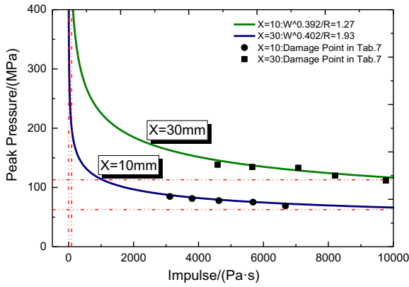
Fig.18 P-I diagrams of cylinder under shock waves in water
