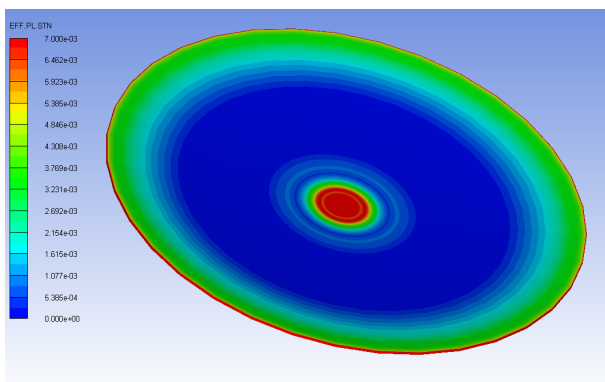
Fig.3 Numerical calculation result of circular plate
