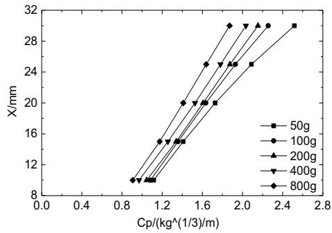
Fig.8 Iso-damage curve of circular plate under peak pressure
