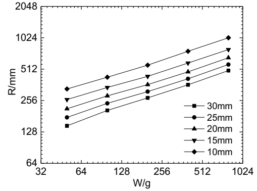
Fig.6 Iso-damage curve of circular plate
