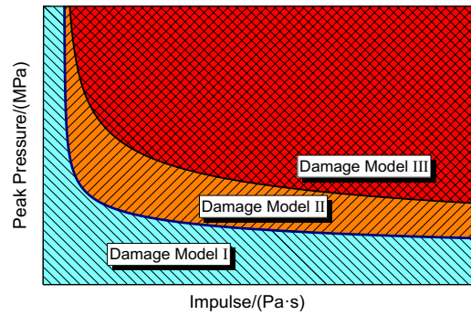
Fig.19 Damage mode based on P-I diagrams
