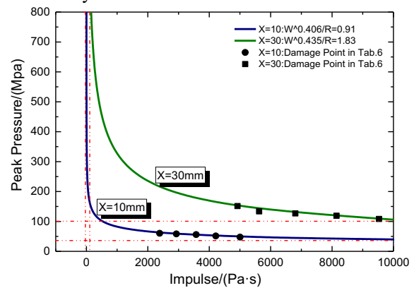
Fig.17 P-I diagrams of circular plate under shock waves in water
