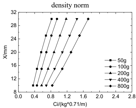
Fig.10 Iso-damage curve of circular plate under impulse norm
