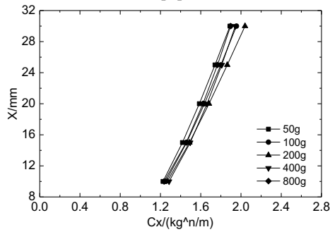
Fig.15 Iso-damage curve of cylinder under damage norm in this paper
