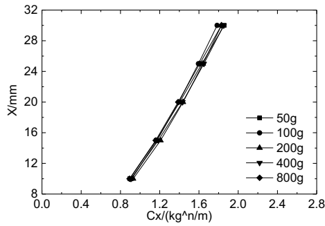
Fig.14 Iso-damage curve of circular plate under damage norm in this paper
