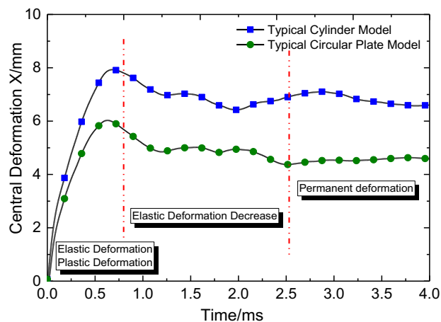
Fig.5 Deformation-time curve of target geometric center
