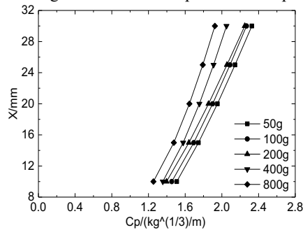
Fig.11 Iso-damage curve of cylinder under peak pressure norm
