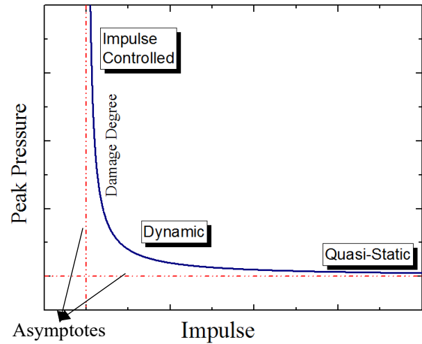
Fig.16 Typical P-I diagrams
