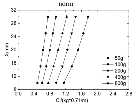
Fig.13 Iso-damage curve of cylinder under impulse norm
