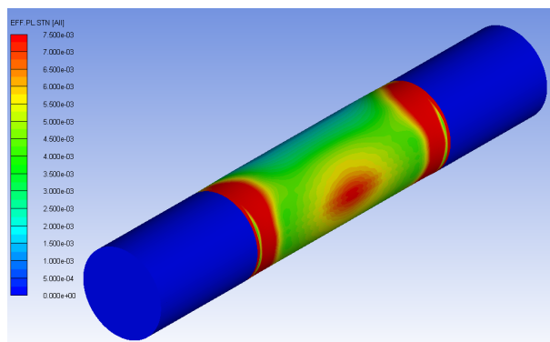
Fig.4 Numerical calculation result of cylinder
