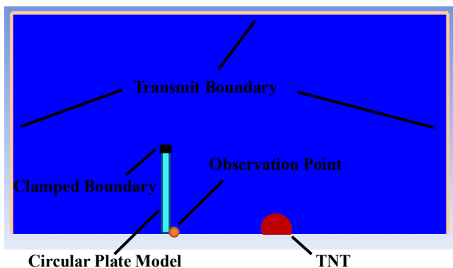
Fig.1 Finite element model of circular plate
