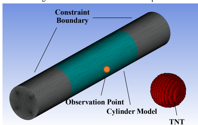
Fig.2 Finite element model of cylinder
