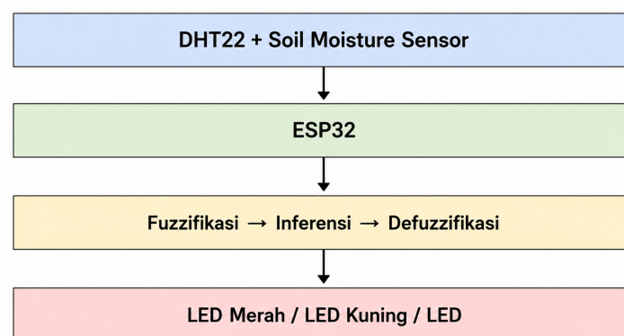
Gambar 7: Diagram blok sistem percobaan
