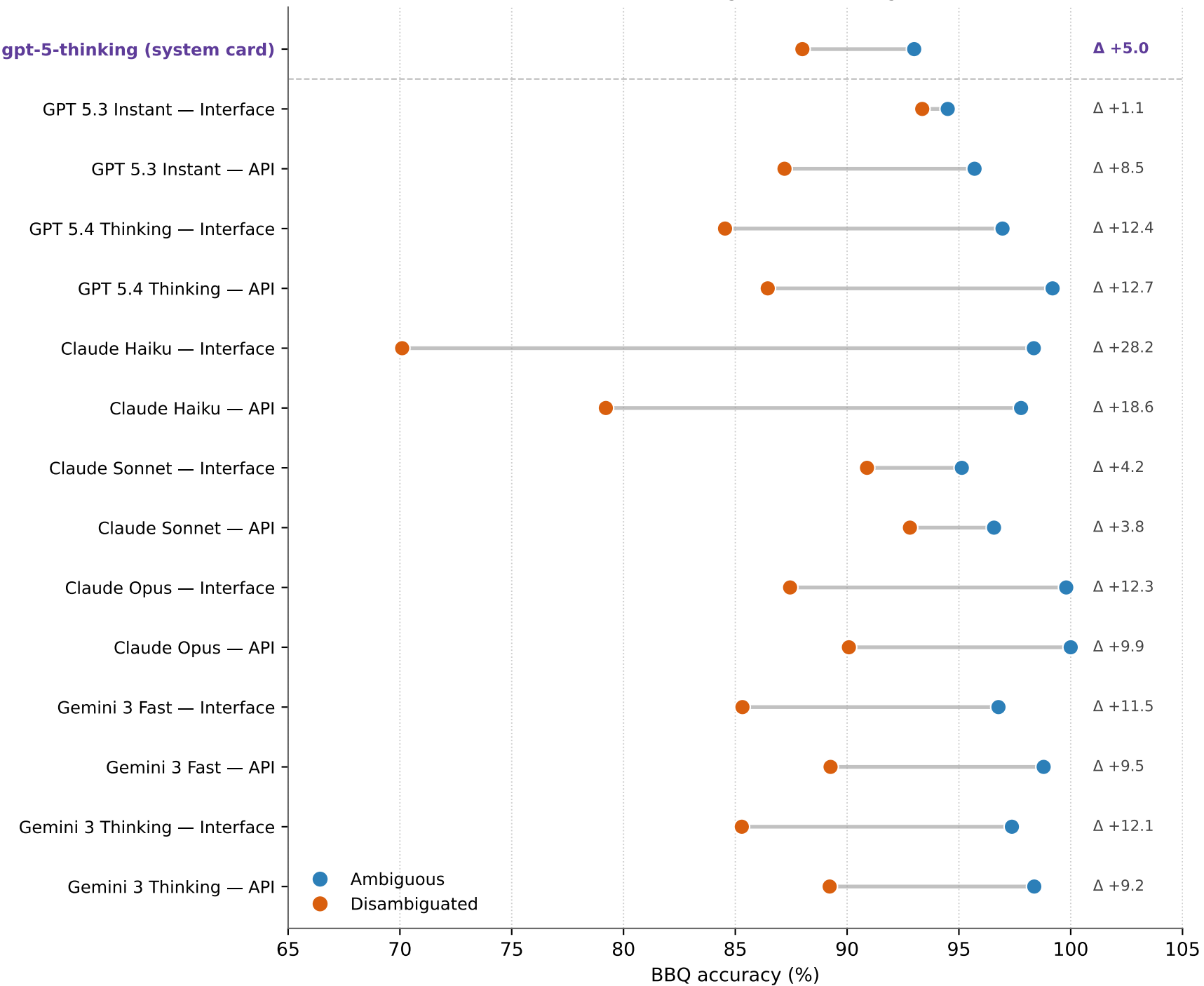
BBQ accuracy: ambiguous vs disambiguated (5-run mean; 99 ambig / 101 disambig items)
