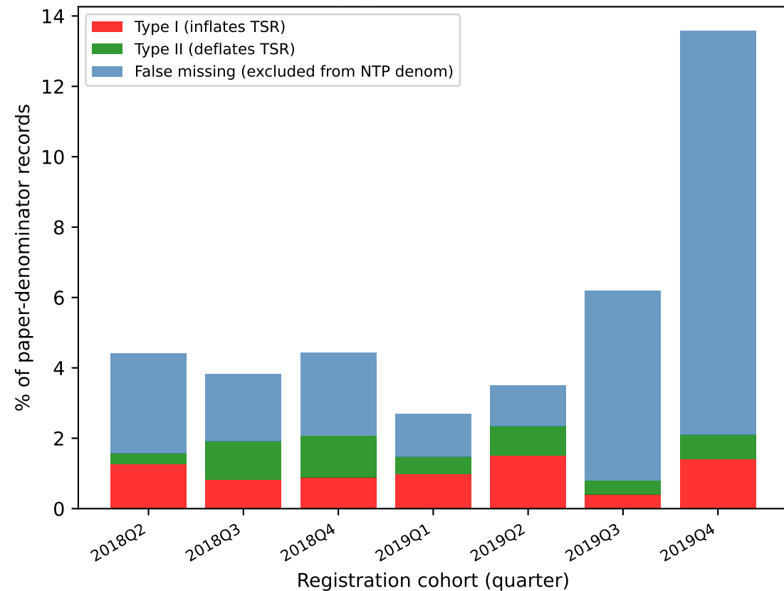
Error composition by registration cohort (% of paper-audited records)
