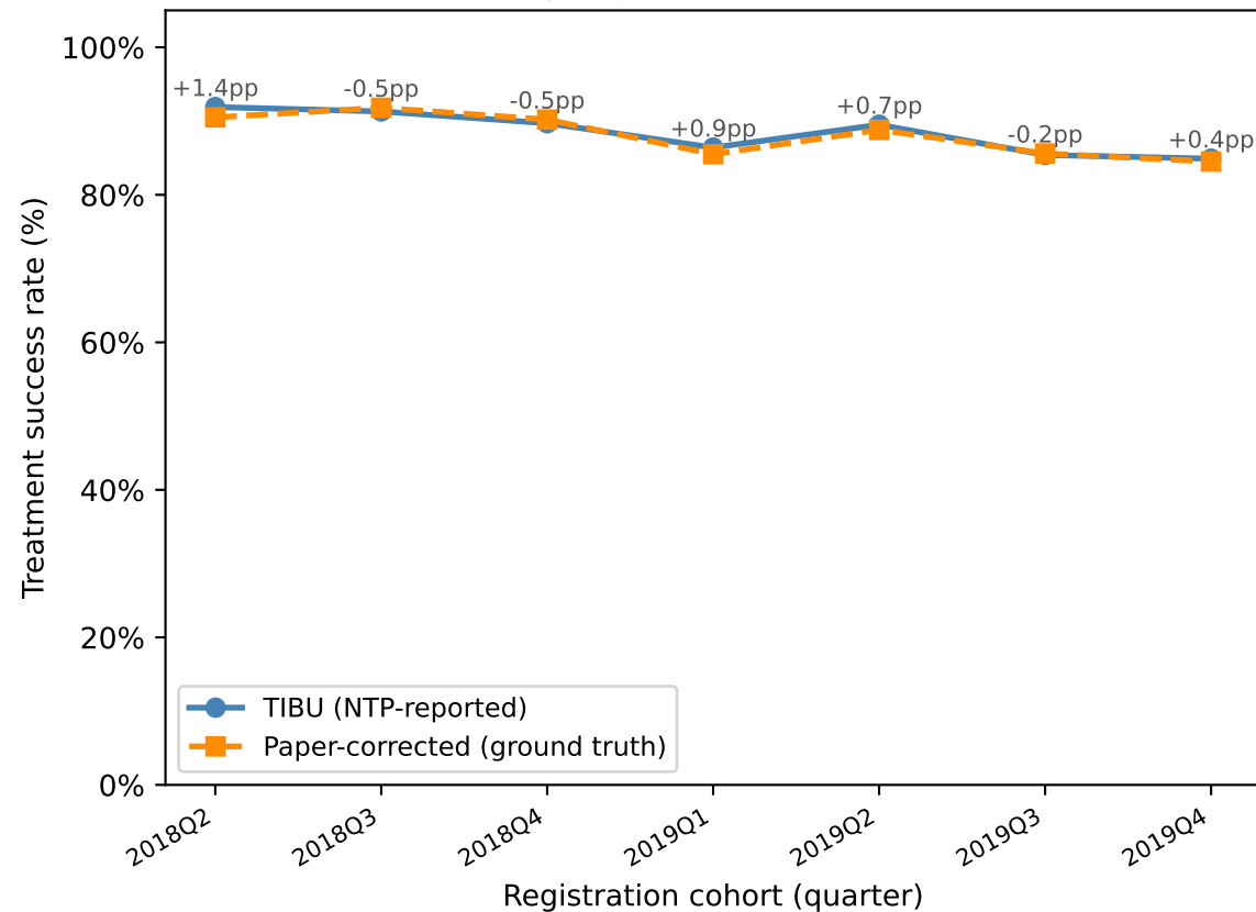
TIBU vs. paper-corrected TSR by registration cohort
