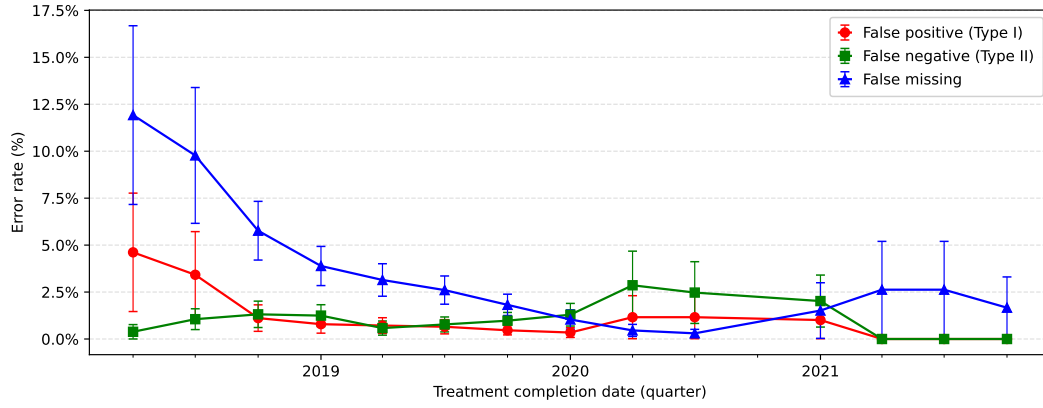
Figure 4: DQA error rates over time, binned by quarter with a 3-quarter centered rolling mean ( N \geq 10 per quarter).
