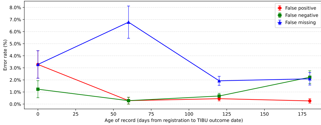
Figure 3: DQA error rates by age of record, restricted to bins with N \geq 100 .
