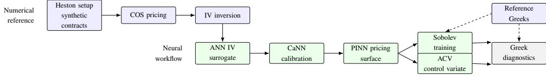
Fig. 1.1. High-level structure of the benchmarked Heston workflow. Solid arrows show the main computational flow; dashed arrows show reference Greeks used to compute diagnostic errors and to define Sobolev Greek targets.
