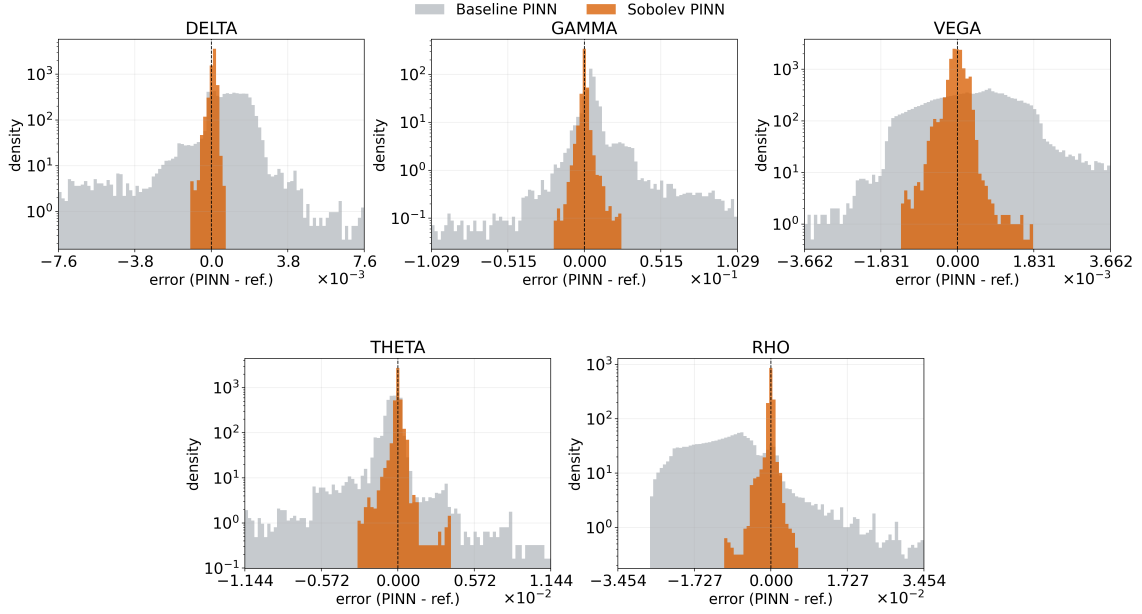
Fig. 5.6. Baseline–Sobolev PINN Greek error histograms. Overlaid density histograms of the pointwise Greek errors summarized in Table 5.8, comparing the baseline PINN with the Sobolev PINN against the Heston Greek reference defined in Section 2.7.2 on the fixed (m, \tau) benchmark grid. The five panels correspond to Delta, Gamma, Vega, Theta, and Rho; the horizontal axis reports the error with sign convention PINN minus reference, and the vertical axis reports density on a logarithmic scale.
