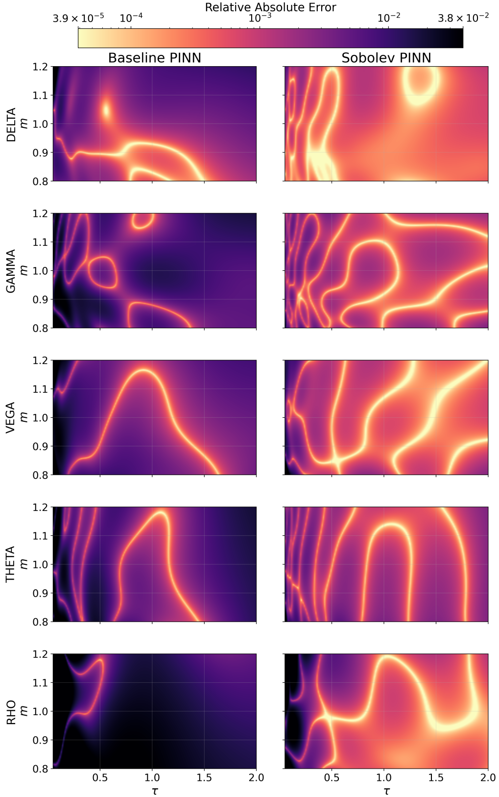
Fig. 5.7. Relative absolute-error maps for PINN-derived Greeks. The two columns compare the baseline PINN and the Sobolev PINN against the Heston Greek reference defined in Section 2.7.2 on the fixed (m, \tau) benchmark grid used for the Greek errors summarized in Table 5.8. Rows correspond to Delta, Gamma, Vega, Theta, and Rho; the horizontal axis is maturity \tau , the vertical axis is moneyness m , and the shared colorbar reports relative absolute error on a logarithmic scale.
