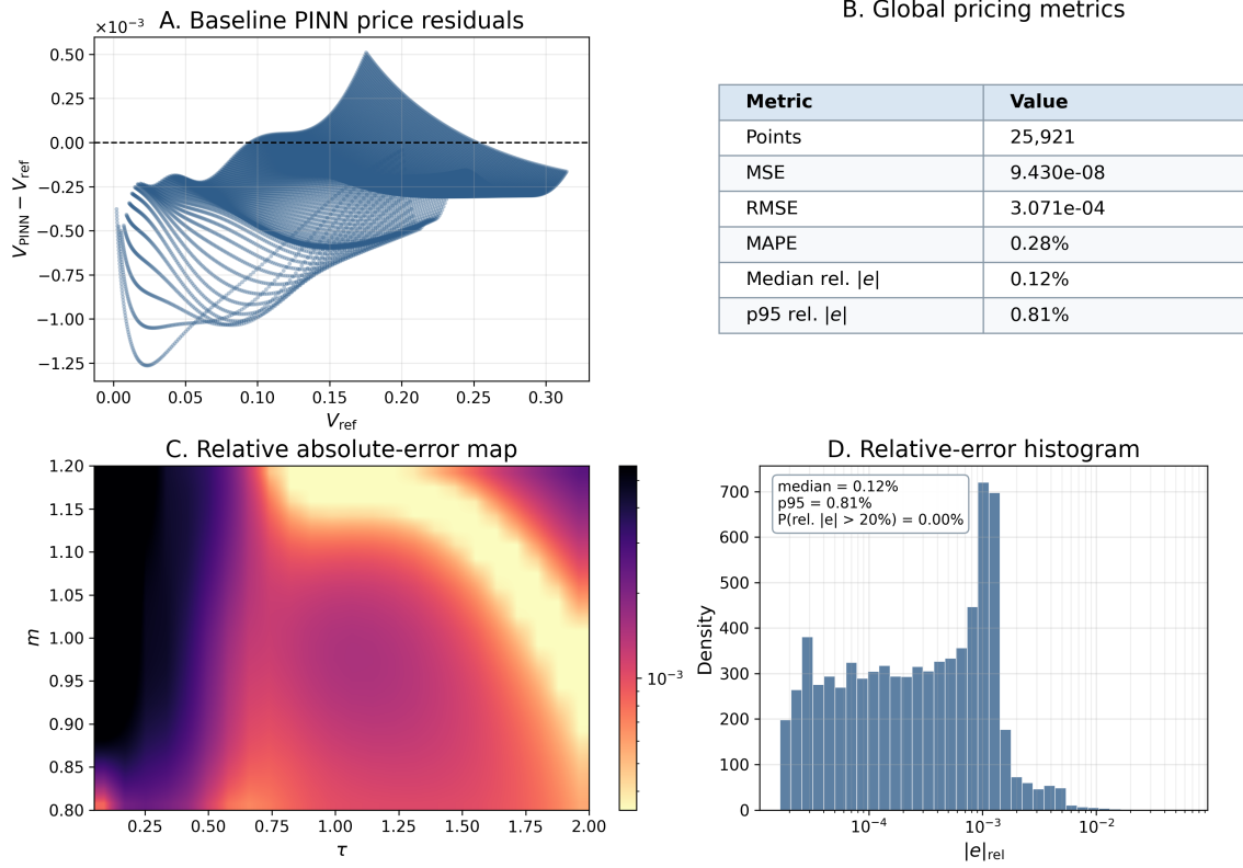
Fig. 5.4. Baseline PINN pricing benchmark versus Heston-COS reference. The baseline PINN is evaluated under the protocol of Appendix B on 25 921 points with m \in [0.8, 1.2] and \tau \in [0.05, 2.0] , using the Heston-COS prices of Section 2.7 as reference. Panel A shows signed price residuals V_{\text{PINN}} - V_{\text{ref}} against V_{\text{ref}} ; Panel B reports the global pricing metrics; Panel C maps the relative absolute pricing error over (\tau, m) ; and Panel D shows its density histogram.
