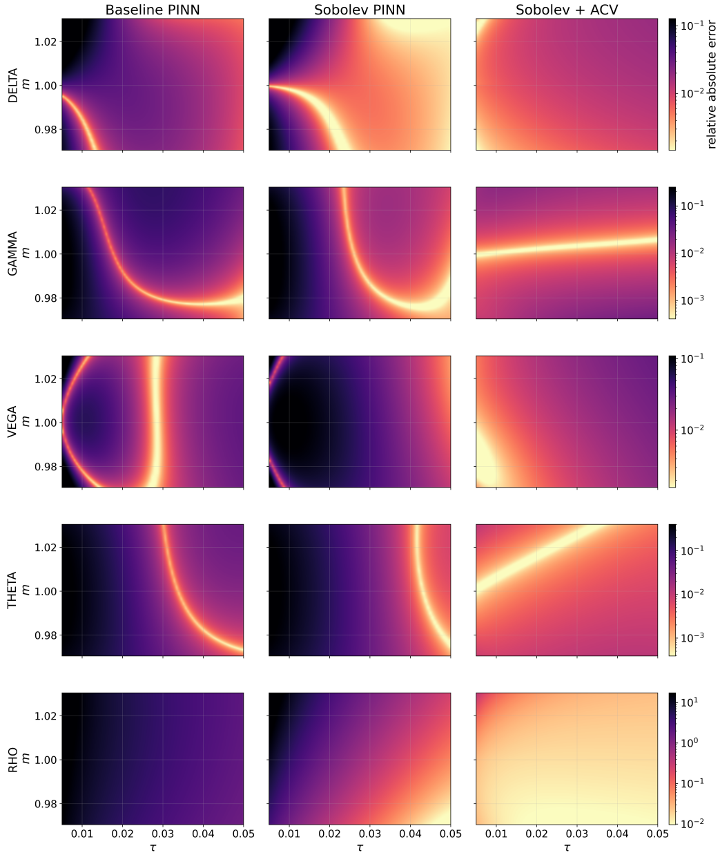
Fig. 5.8. Relative absolute-error maps for PINN-derived Greeks in the short-maturity ATM region. The three columns compare the baseline PINN, the Sobolev PINN, and the Sobolev+ACV correction of Section 4.6 against the Heston Greek reference defined in Section 2.7.2 on the local grid m \in [0.9704, 1.0305] , \tau \in [0.005, 0.05] , corresponding to the hard region of Equation (4.21). Rows correspond to Delta, Gamma, Vega, Theta, and Rho; the horizontal axis is maturity \tau , the vertical axis is moneyness m , and each row uses an independent logarithmic colorbar for the relative absolute error of that Greek.
