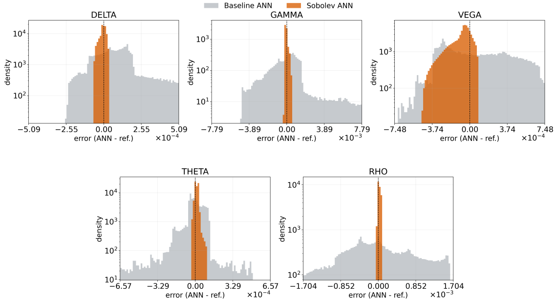
Fig. 5.2. Baseline–Sobolev ANN Greek error histograms. Overlaid density histograms of the pointwise Greek errors summarized in Table 5.3, comparing the ANN baseline with the ANN Sobolev surrogate against the Heston Greek reference defined in Section 2.7.2 on the fixed (m, \tau) benchmark grid. The five panels correspond to Delta, Gamma, Vega, Theta, and Rho; the horizontal axis reports the error with sign convention ANN minus reference, and the vertical axis reports density on a logarithmic scale.
