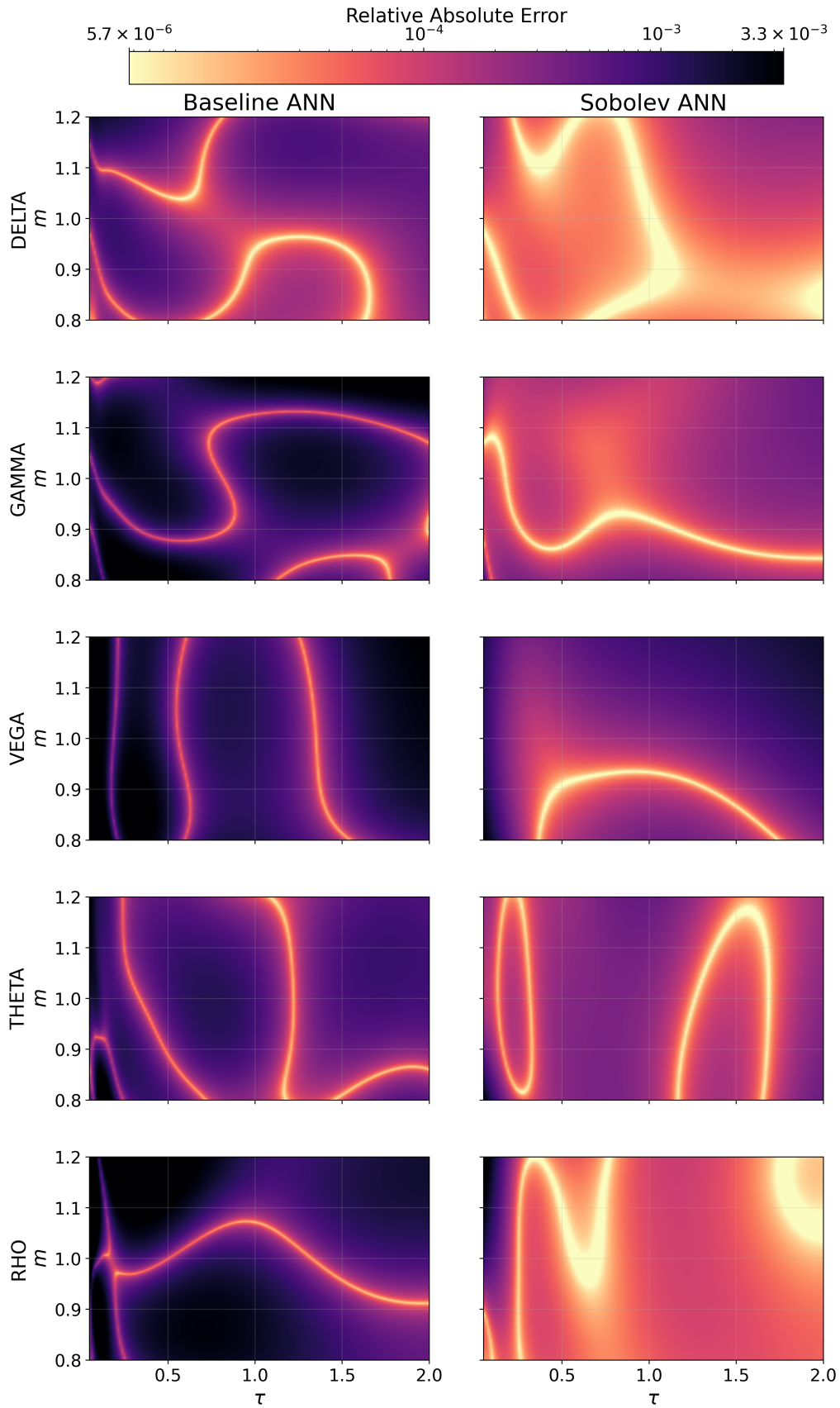
Fig. 5.3. Relative absolute-error maps for ANN-derived Greeks. The two columns compare the ANN baseline and the ANN Sobolev surrogate against the Heston Greek reference defined in Section 2.7.2 on the fixed (m, \tau) benchmark grid used for the Greek errors summarized in Table 5.3. Rows correspond to Delta, Gamma, Vega, Theta, and Rho; the horizontal axis is maturity \tau , the vertical axis is moneyness m , and the shared colorbar reports relative absolute error on a logarithmic scale.
