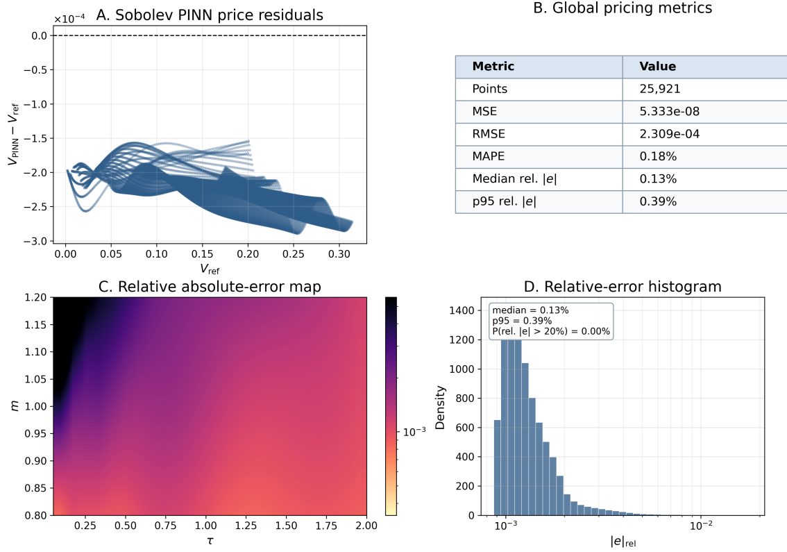
Fig. 5.5. Sobolev PINN pricing benchmark versus Heston-COS reference. The Sobolev PINN of Section 4.5 is evaluated under the protocol of Appendix B on 25 921 points with m \in [0.8, 1.2] and \tau \in [0.05, 2.0] , using the Heston-COS prices of Section 2.7 as reference. Panel A shows signed price residuals V_{\text{PINN}} - V_{\text{ref}} against V_{\text{ref}} ; Panel B reports the global pricing metrics; Panel C maps the relative absolute pricing error over (\tau, m) ; and Panel D shows its density histogram.
