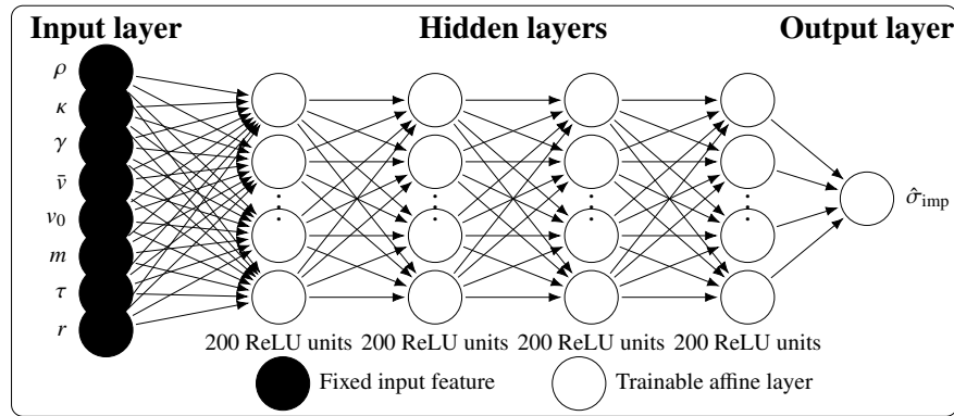
Fig. 3.1. Fully connected ANN pricer used in the forward Heston implied-volatility surrogate. The eight fixed inputs are mapped through four hidden layers of width 200, and the final linear layer returns the predicted implied volatility.
