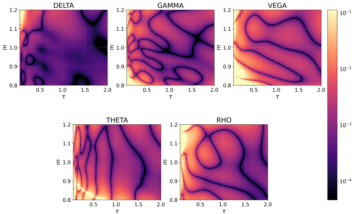
Fig. 6.5. Sobolev PINN Greek relative-error maps.
