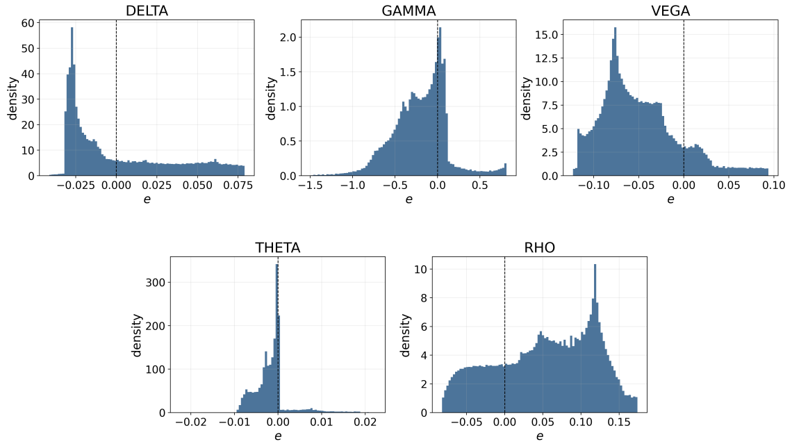
Fig. 5.8. Baseline PINN Greek error histograms.
