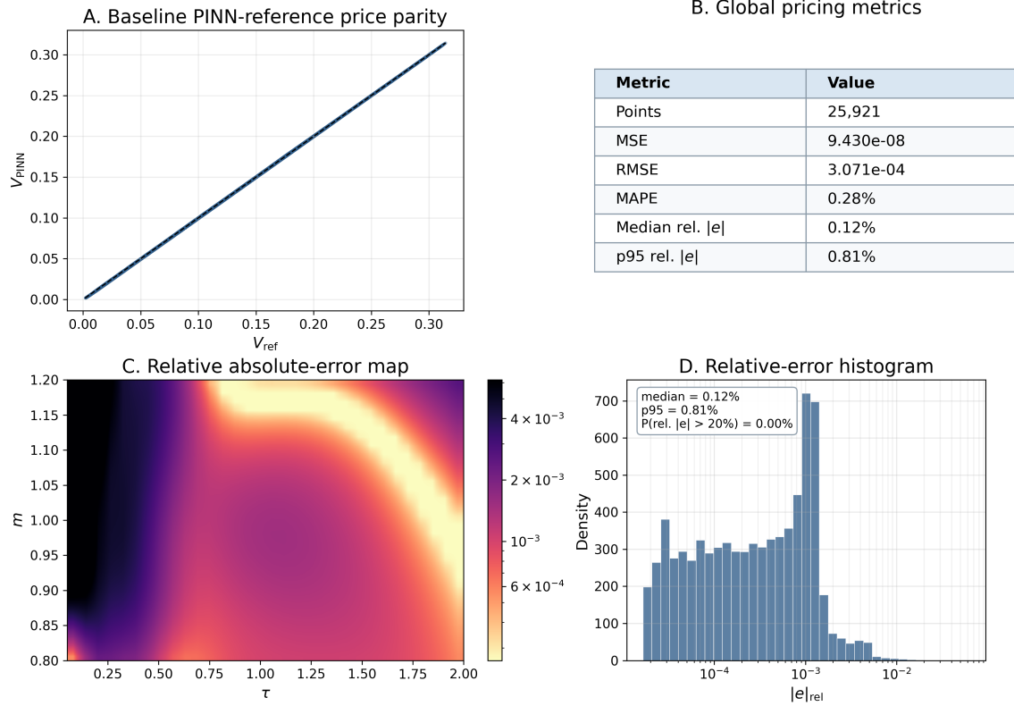
Fig. 5.3. Baseline PINN pricing benchmark versus reference. Top-left: PINN-reference scatter. Top-right: global MSE/RMSE/MAPE and relative-error summary. Bottom-left: mean relative absolute-error map over (\tau, m) , with the color scale representing the cellwise mean relative absolute error. Bottom-right: histogram of relative absolute pricing errors.
