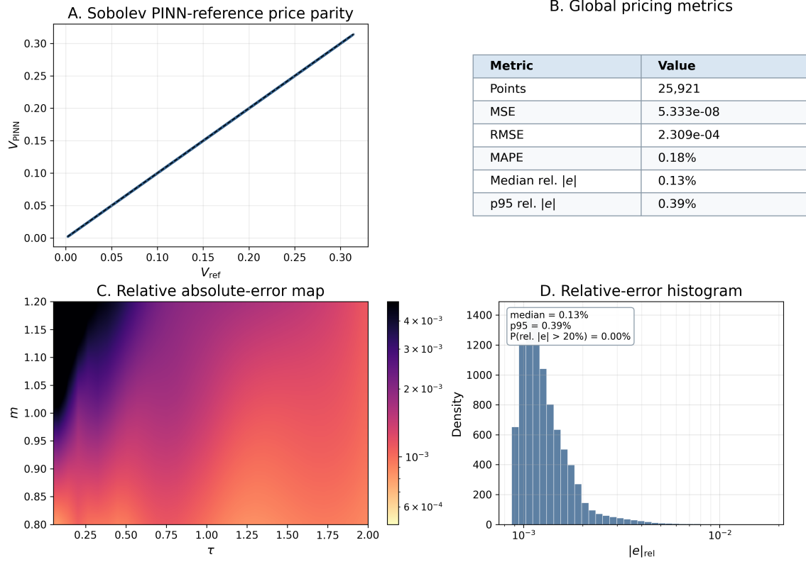
Fig. 5.4. ADAPTAR. Sobolev PINN pricing benchmark versus reference. The panels follow the same layout as Figure 5.3; in the spatial panel, the color scale represents the cellwise mean relative absolute error over (\tau, m) .
