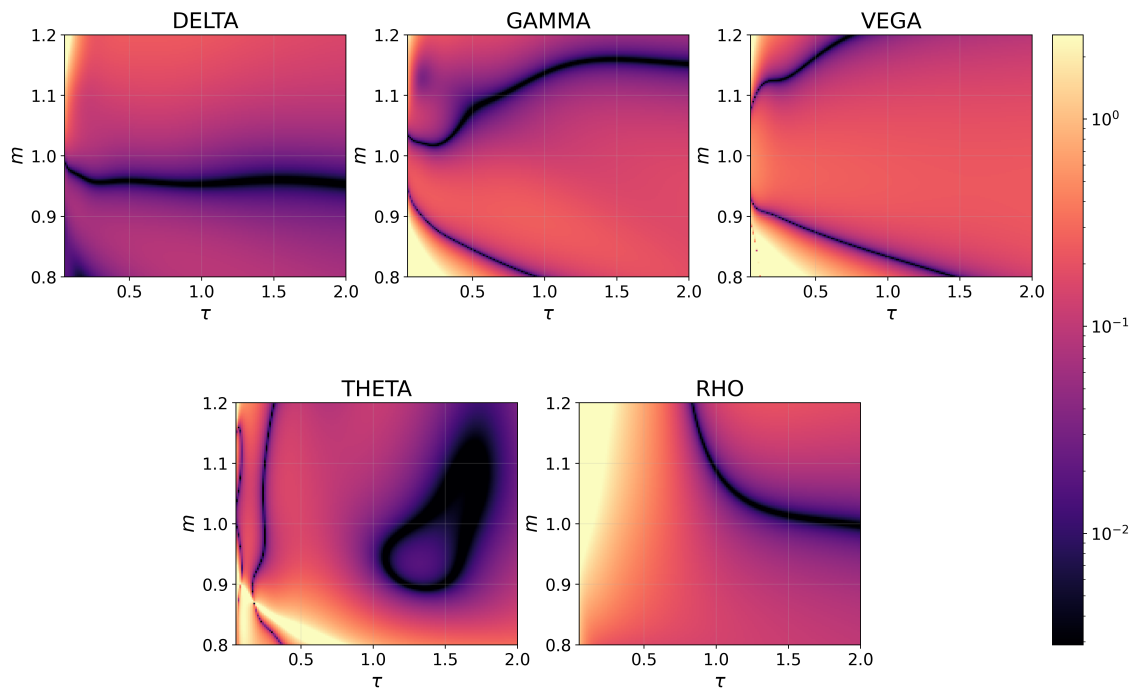
Fig. 5.6. Baseline PINN Greek relative-error maps.
