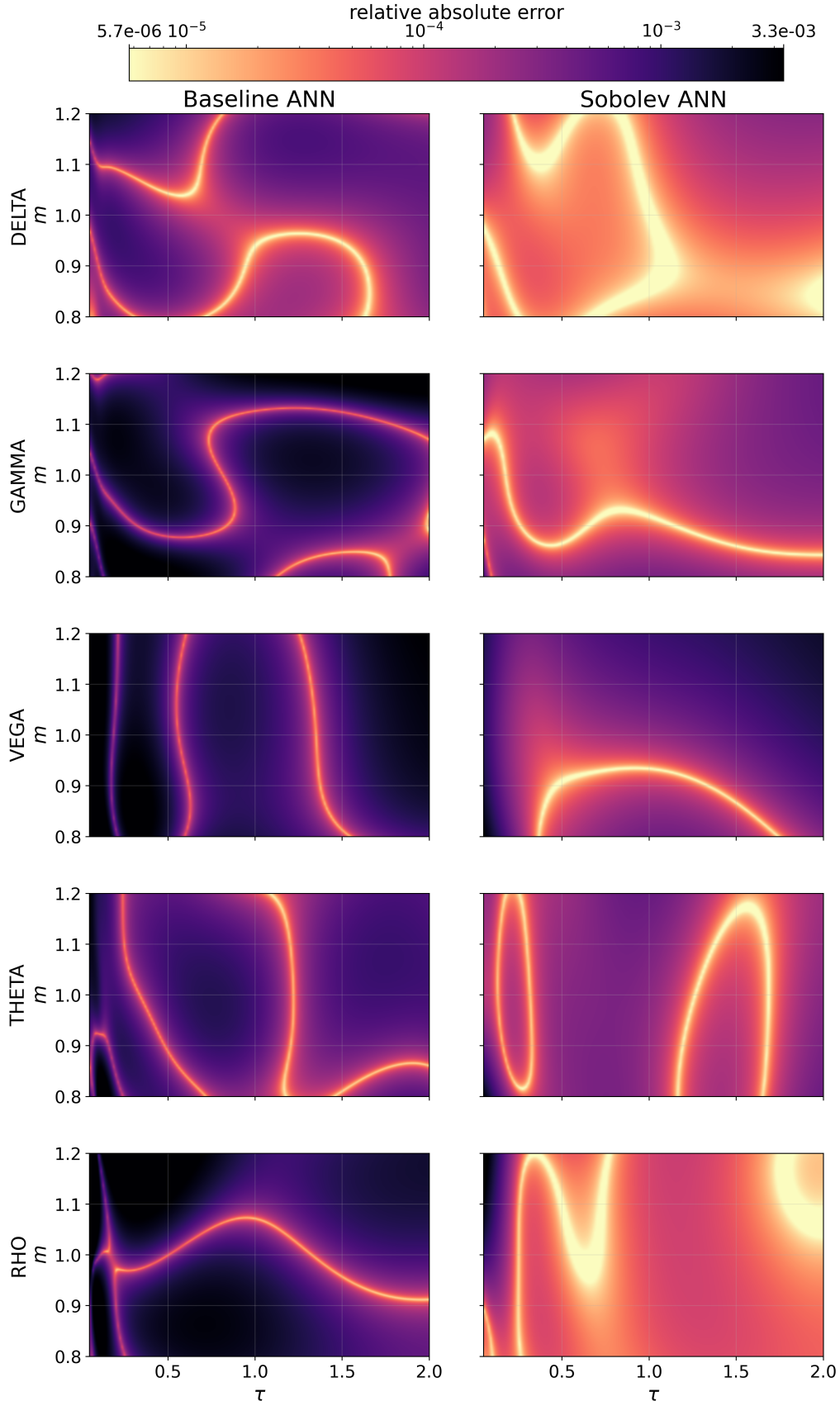
Fig. 5.2. Relative absolute-error maps for ANN-derived Greeks. For each Greek, the baseline ANN and the ANN Sobolev surrogate are evaluated on the same fixed (m, \tau) grid against the Heston characteristic-function reference. Sobolev training visibly contracts the high-error regions and gives a more homogeneous sensitivity surface, especially for GAMMA, RHO, and DELTA.
