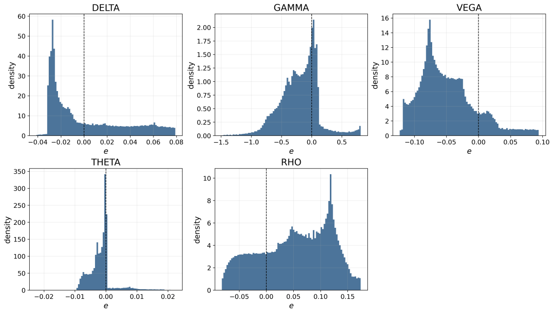
Fig. 6.8. Baseline PINN Greek error histograms.
