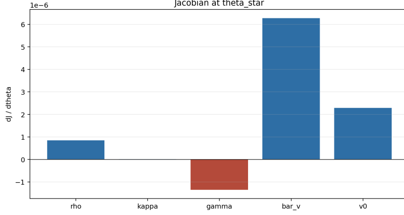
Fig. 4.6. Objective-gradient components at \theta^* for the selected no-regularization calibration. Near-zero components support first-order stationarity of the selected solution.
