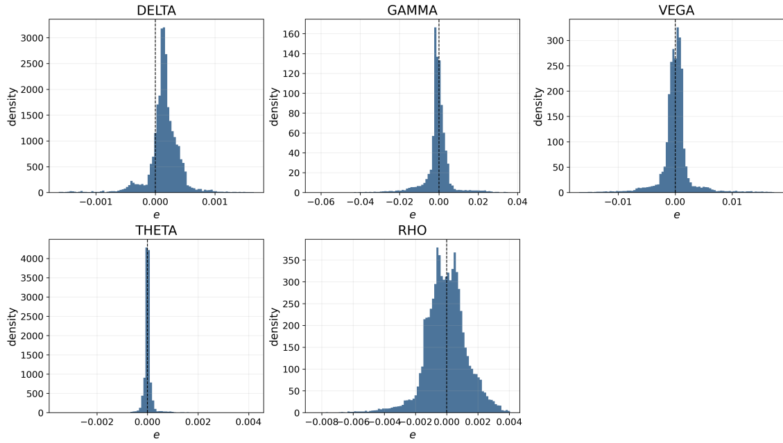
Fig. 6.10. Sobolev PINN Greek error histograms.
