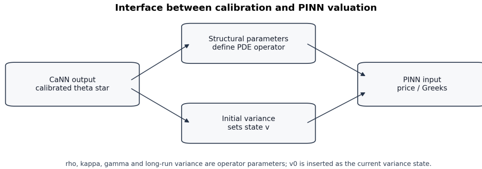
Fig. 4.8. Interface between the calibrated Heston vector and the downstream PINN input convention. Structural parameters define the PDE operator, while v_0^* is used as the variance-state coordinate at market evaluation.
