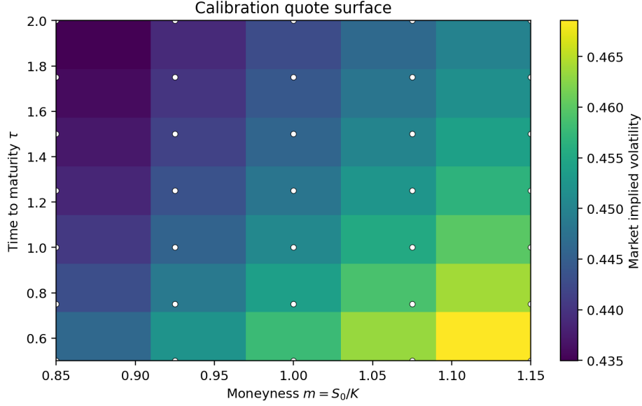
Fig. 4.2. Implied-volatility surface used as calibration input in the Liu-style synthetic experiment. Markers show the 35 observed quote locations.
