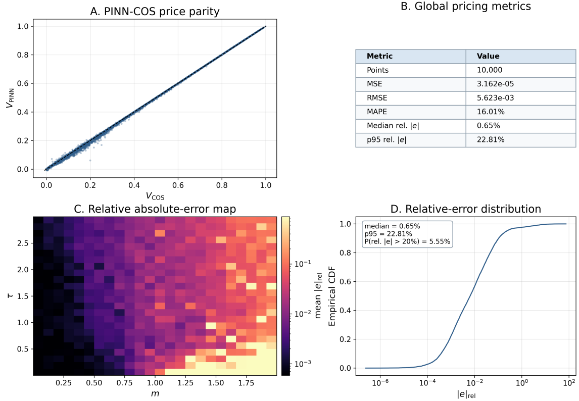
Fig. 6.6. Composite PINN pricing benchmark versus COS reference. Top-left: PINN-COS scatter. Top-right: global MSE/RMSE/MAPE and relative-error summary. Bottom-left: mean relative absolute-error map over (m, \tau) . Bottom-right: empirical CDF of relative absolute pricing errors.
