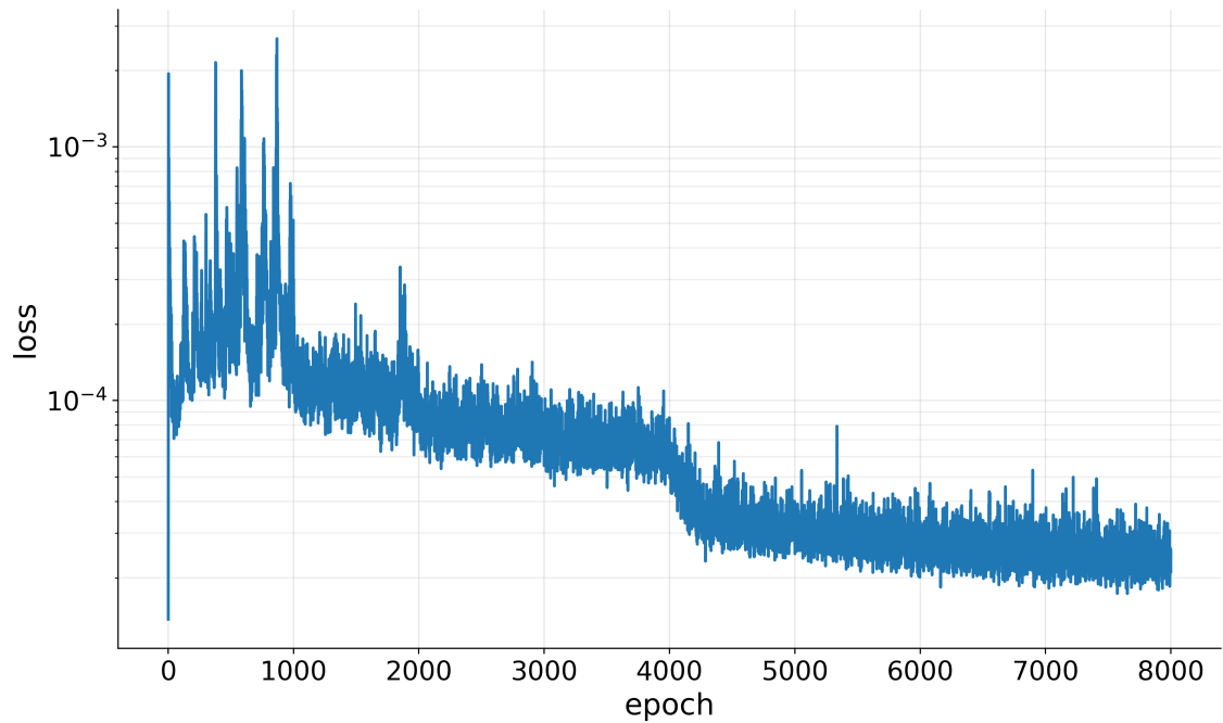
Fig. 6.11. Training loss trajectory with phase switch at epoch 4000 (without Sobolev before 4000, with Sobolev from 4000 onward).
