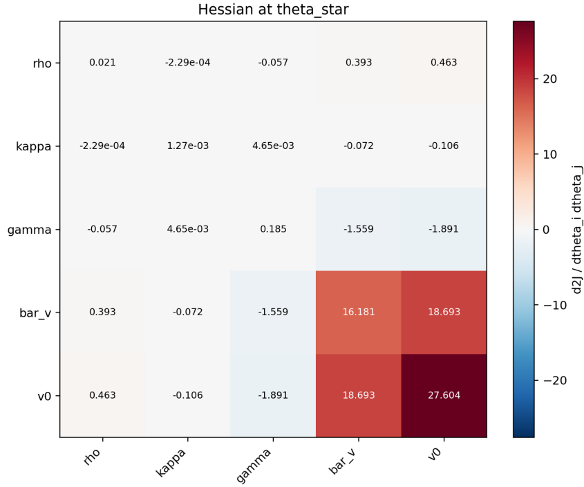
Fig. 4.7. Hessian matrix at \theta^* for the selected no-regularization calibration. The variance block around (\bar{v}, v_0) is locally stiffer than the remaining directions, indicating uneven parameter identifiability.
