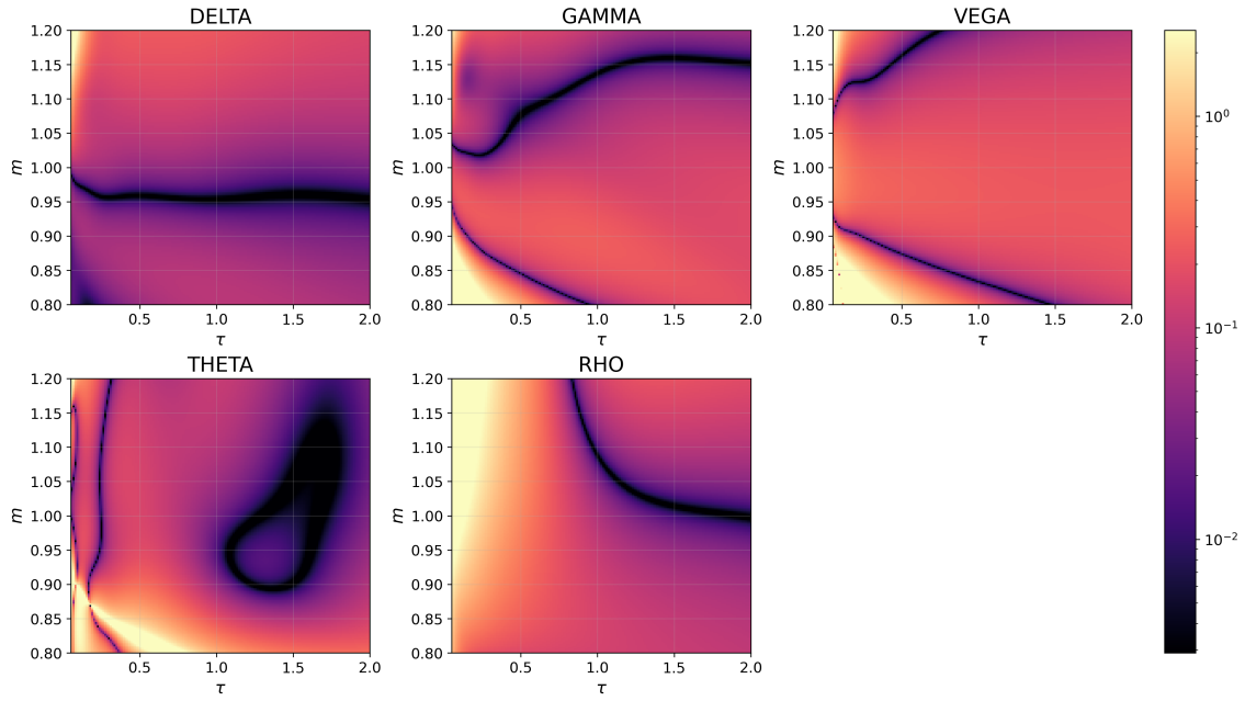
Fig. 6.7. Baseline PINN Greek relative-error maps.
