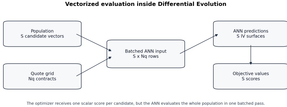
Fig. 4.3. Vectorized population evaluation used inside the calibration loop. Candidate parameters are crossed with the quote grid, scored as implied-volatility surfaces, and returned to the optimizer as one objective value per candidate.
