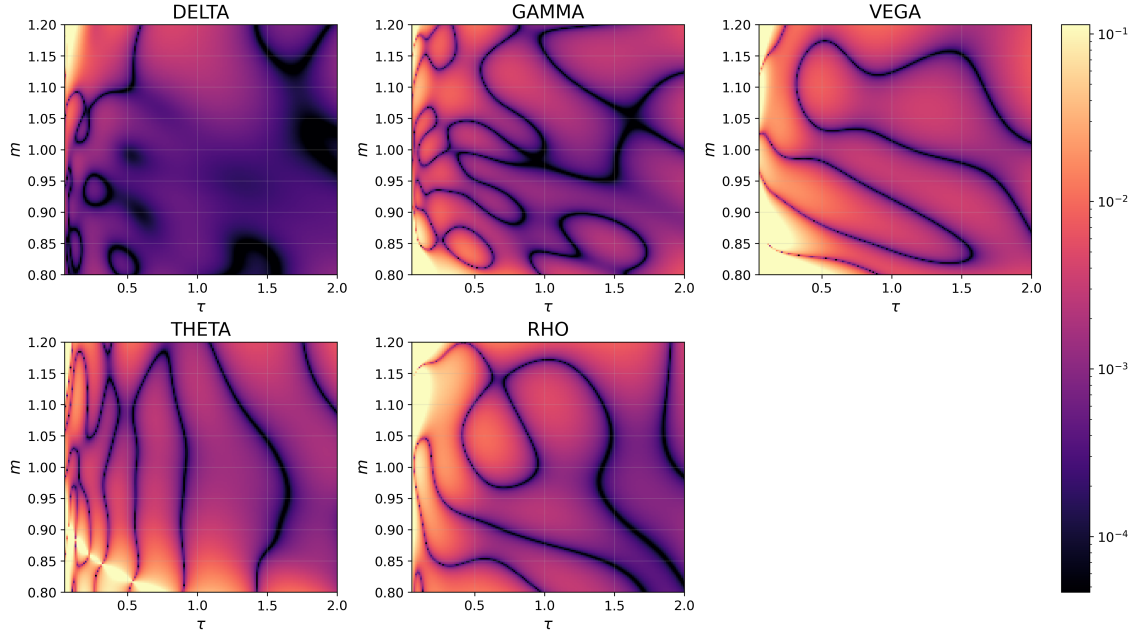
Fig. 6.9. Sobolev PINN Greek relative-error maps.
