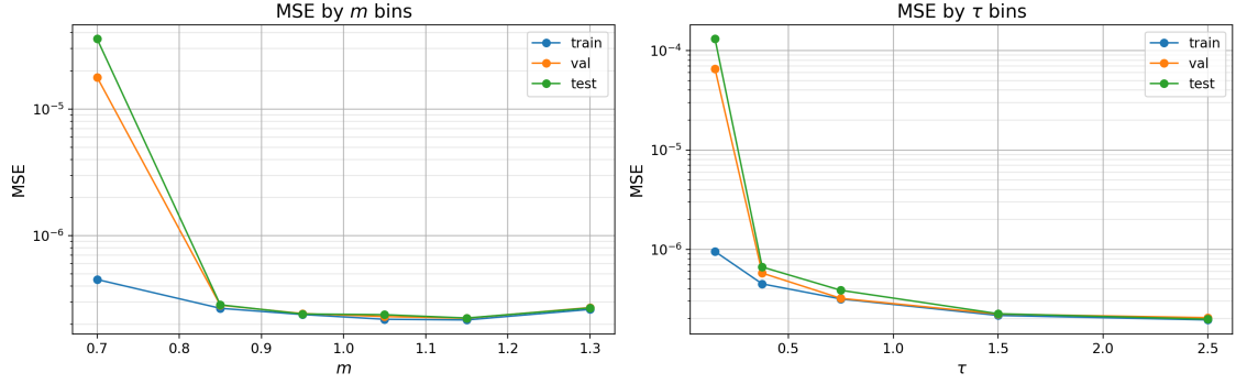
Fig. 6.2. Regional ANN MSE by moneyness bins (left) and maturity bins (right). Curves correspond to train, validation, and test.
