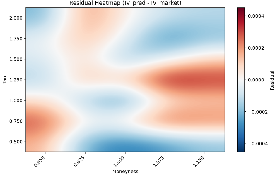
Fig. 4.5. Signed implied-volatility residual map for the selected CaNN calibration, defined as IV_{\text{pred}} - IV_{\text{market}} . The smoothing is visual only; the calibration is performed on the original quote grid.
