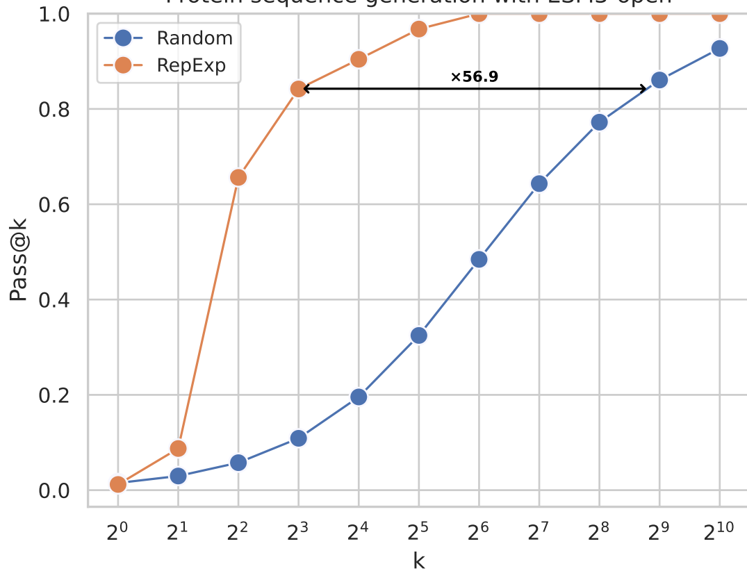
Protein sequence generation with ESM3-open
