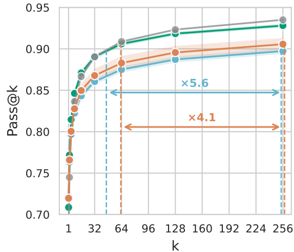
MATH
