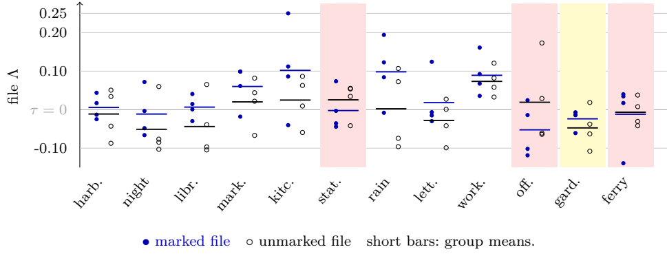
Yellow (garden): ranking win, 0/4 marked files above \tau . Rose (station, office, ferry-queue): ranking loss with isolated TPs.
