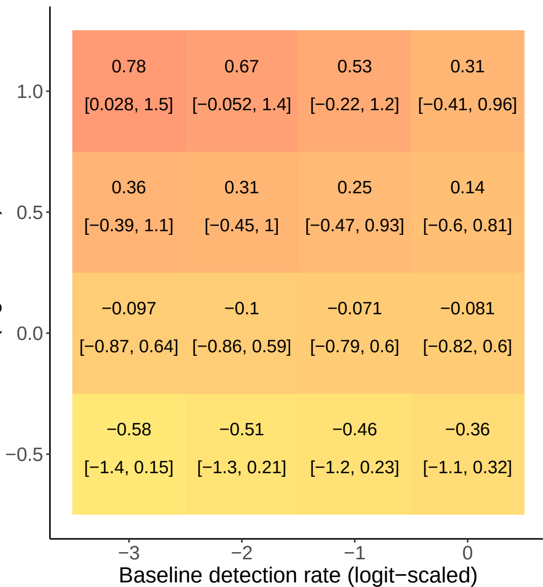
Effect of habitat on detection rate (logit-scaled)
