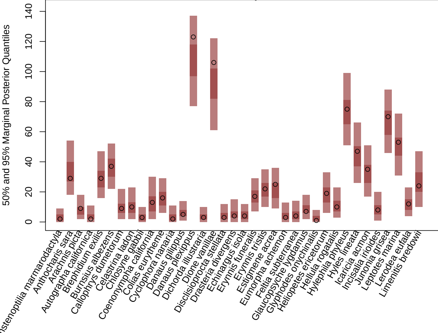
Real Detections vs. Model Expectations of Detections
