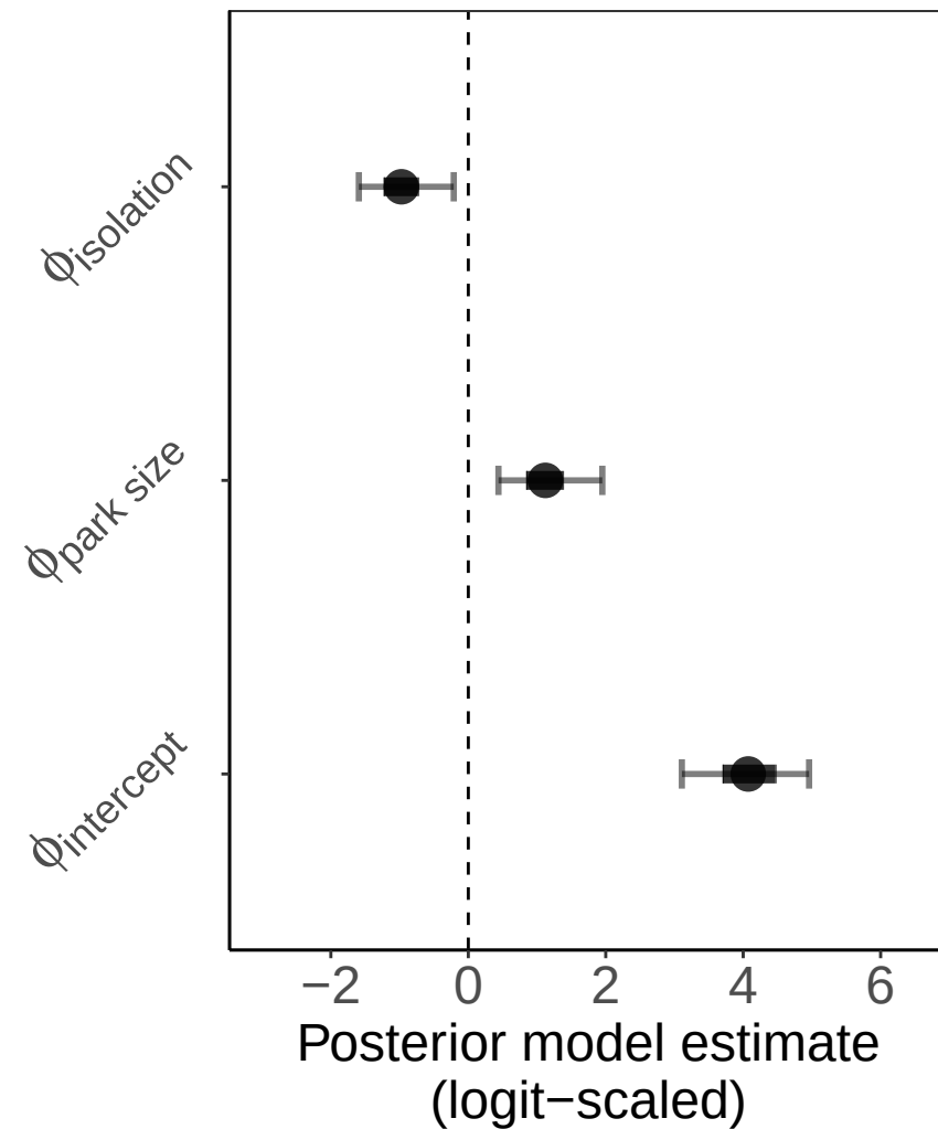
c) Persistence
