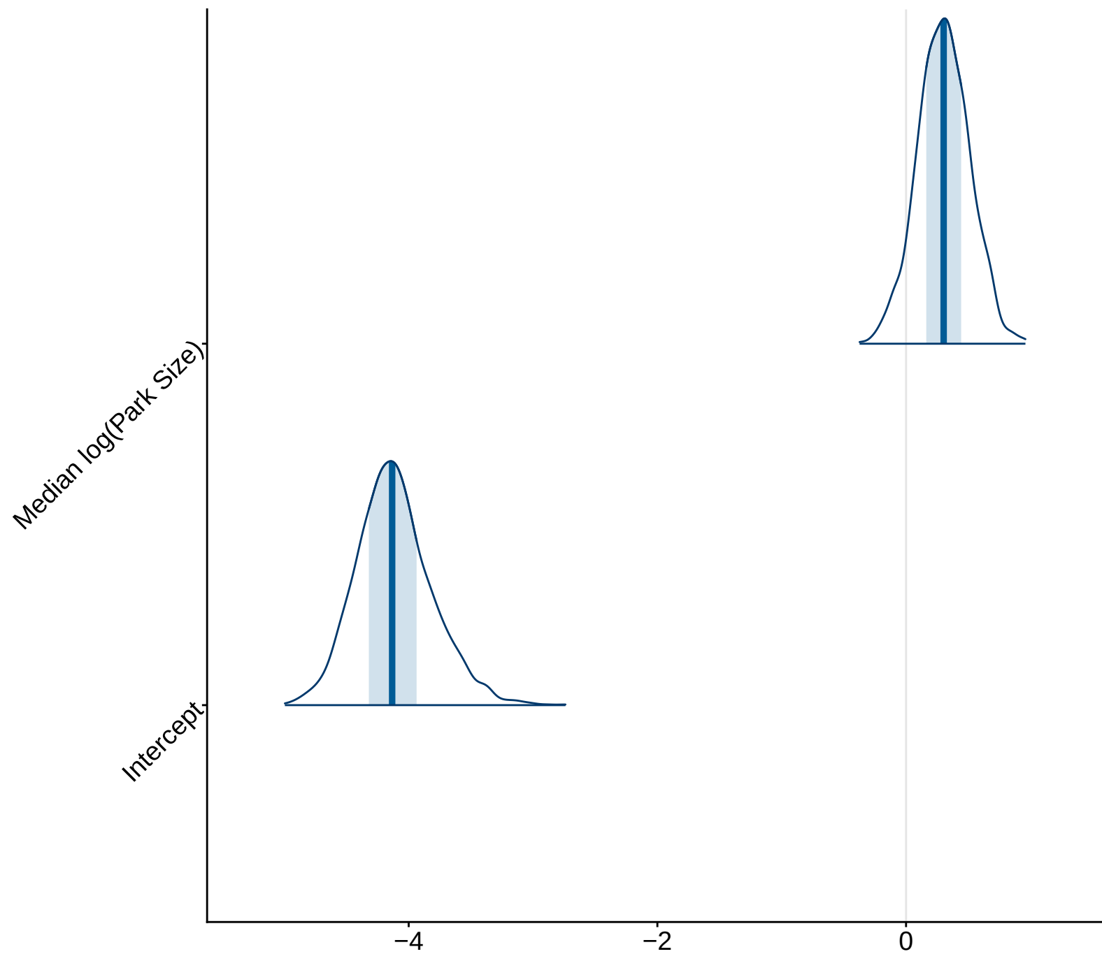
Posterior densities of sampled parameters from models fit to 100 simulated communities
