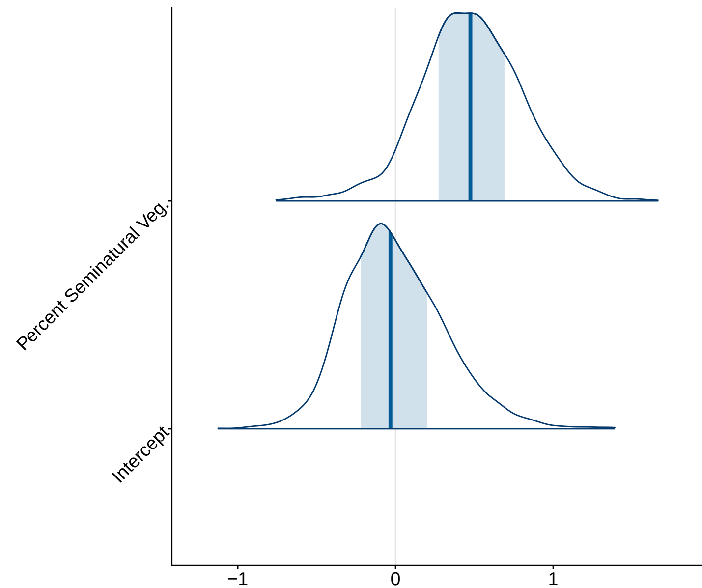
Posterior densities of sampled parameters from models fit 100 simulated communities
