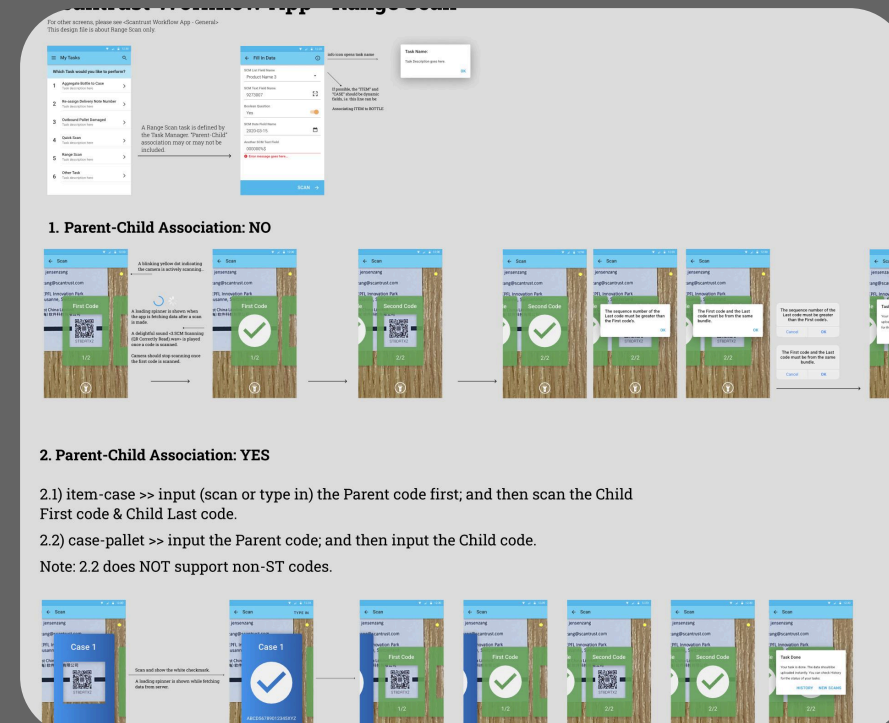
Supply Chain App - Warehouse
