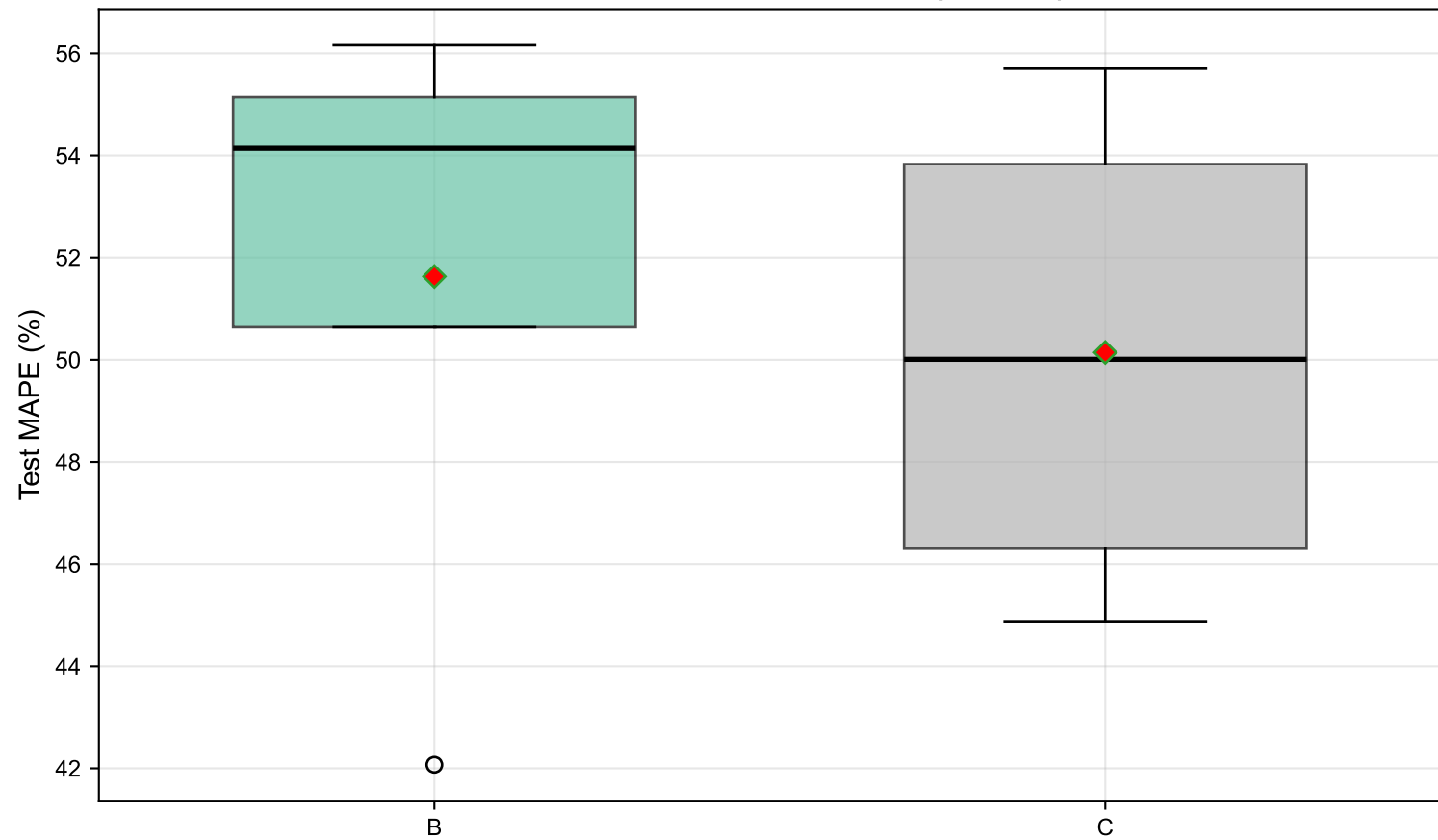
Multi-Seed Experiment Results (5 seeds)
