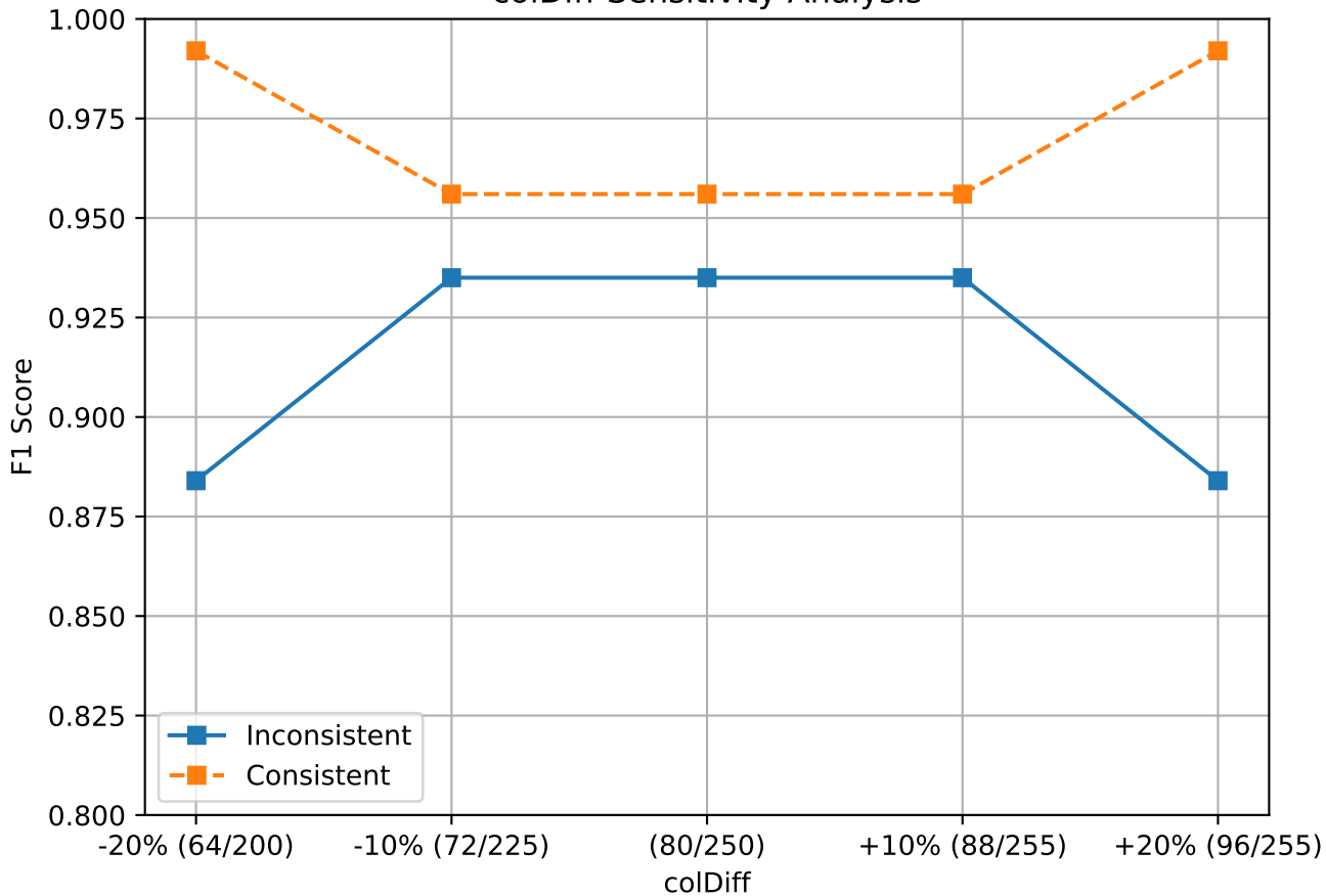
colDiff Sensitivity Analysis
