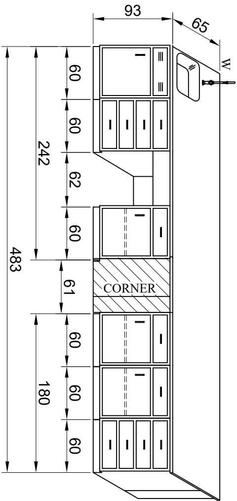
ELEVATION 'A'
