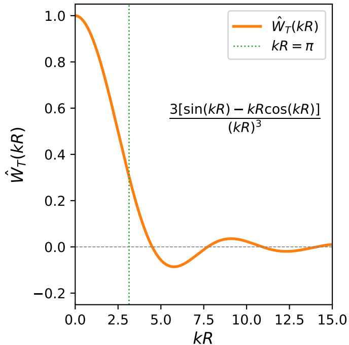
Fourier space
