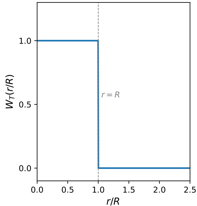
Real space
