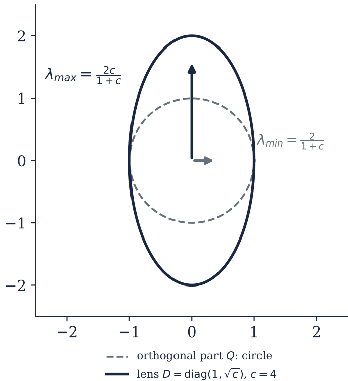
2D elliptic carrier W = D^{-1}R(\theta)D
