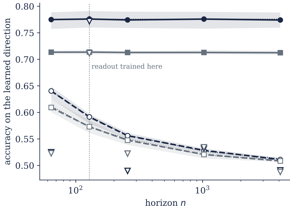
Isolated storage preserves accuracy; the frozen readout ages
