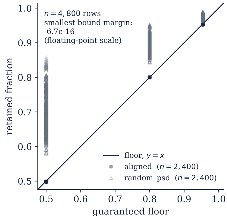
Approximate isolation: retention and its lower bound
