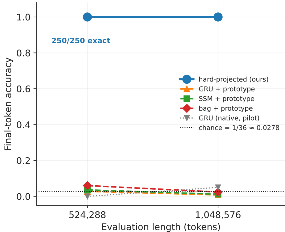
(b) Million-token regime
