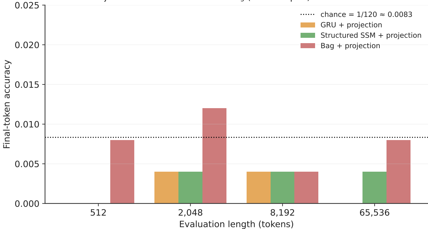
Projection-matched baselines on S_5 (held-out-pair): all near chance
