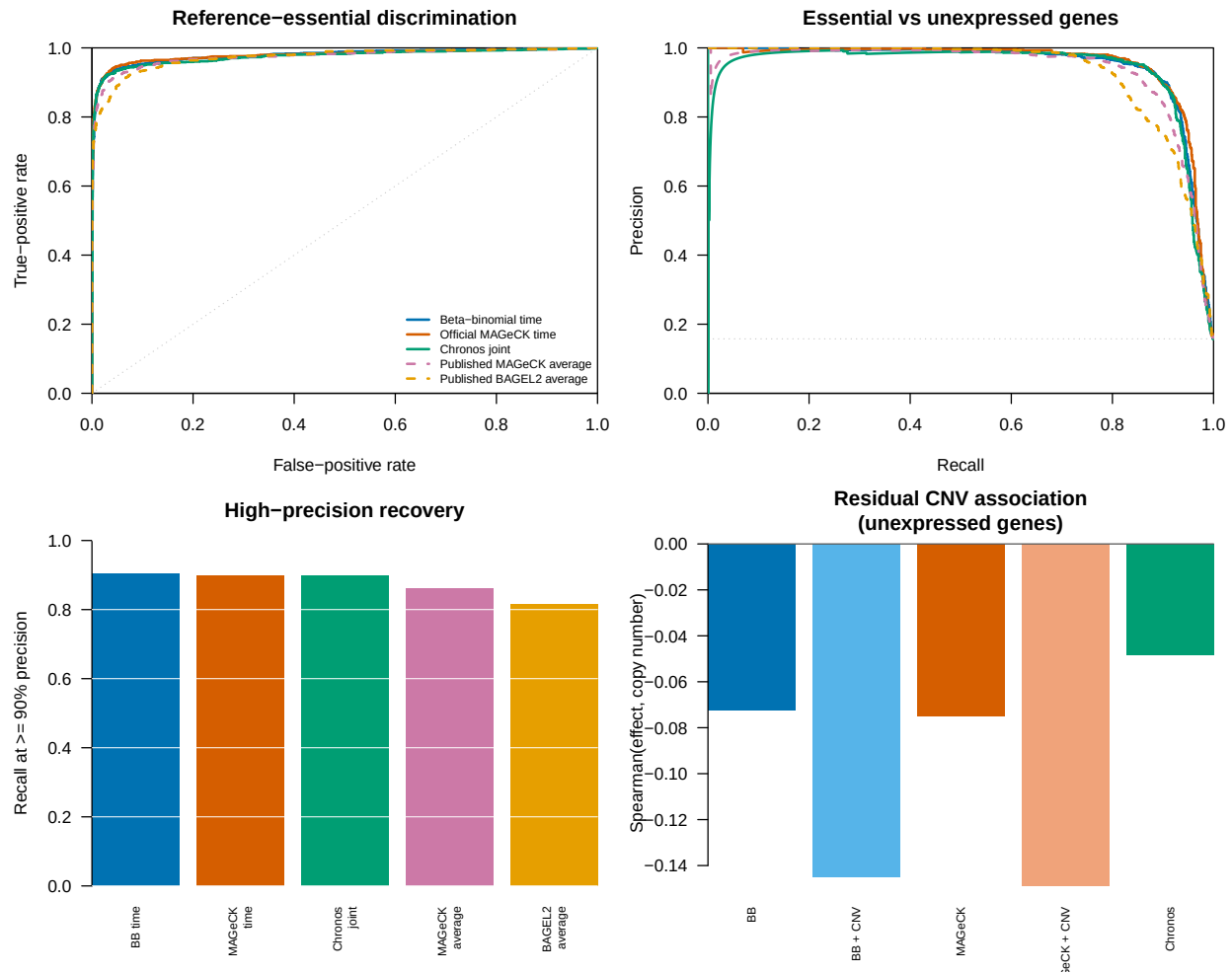
Figure 1: Longitudinal HT-29 benchmark. The upper panels compare control-gene ROC and precision–recall curves. The lower-left panel shows recall at at least 90% precision. The lower-right panel shows residual effect–copy-number association among unexpressed genes before and after official MAGECK piecewise correction; the more negative corrected bars demonstrate over-correction in this single-cell-line screen.
