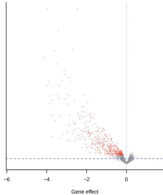
MAGeCK-MLE
