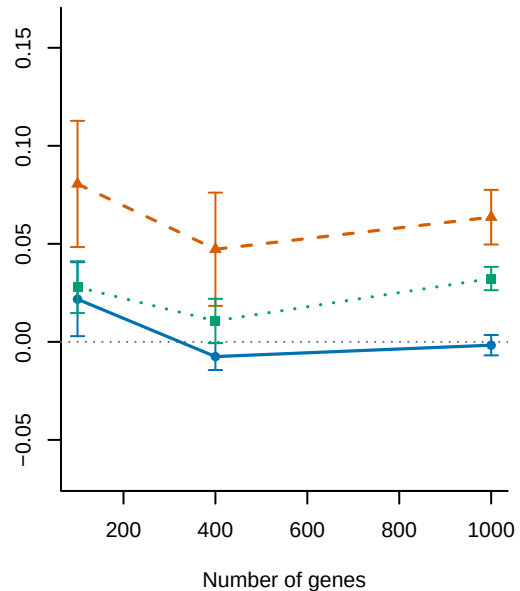
C Number of genes
