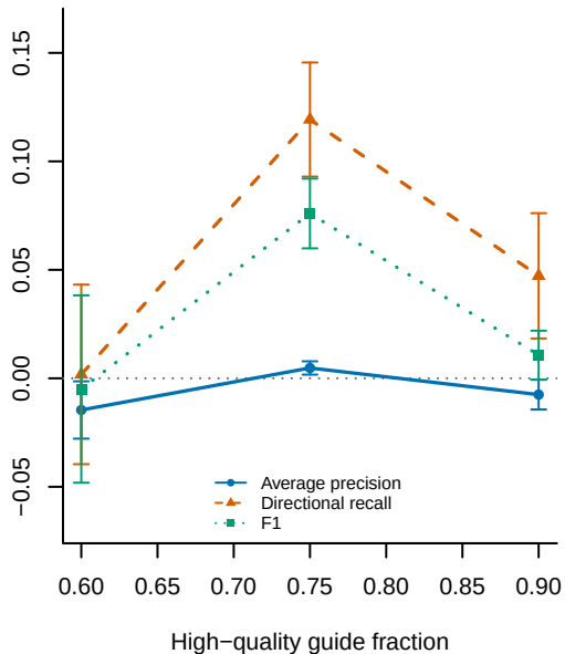
B High-quality guide fraction
